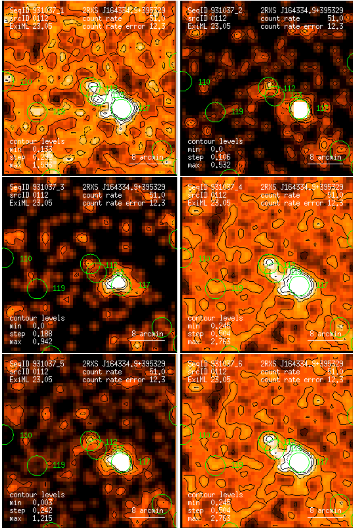
Figure 112: RASS 931037: detection 0112: band rate images, Gaussian filter: (1) PSPC channels 11 – 41, (2) 52 – 90, (3) 91 – 201, (4) 11 – 235, (5) 52 – 201, (6) 11 – 201. Broad band rates in counts/ks. Band rate contour levels in counts/ks/arcmin 2 .
