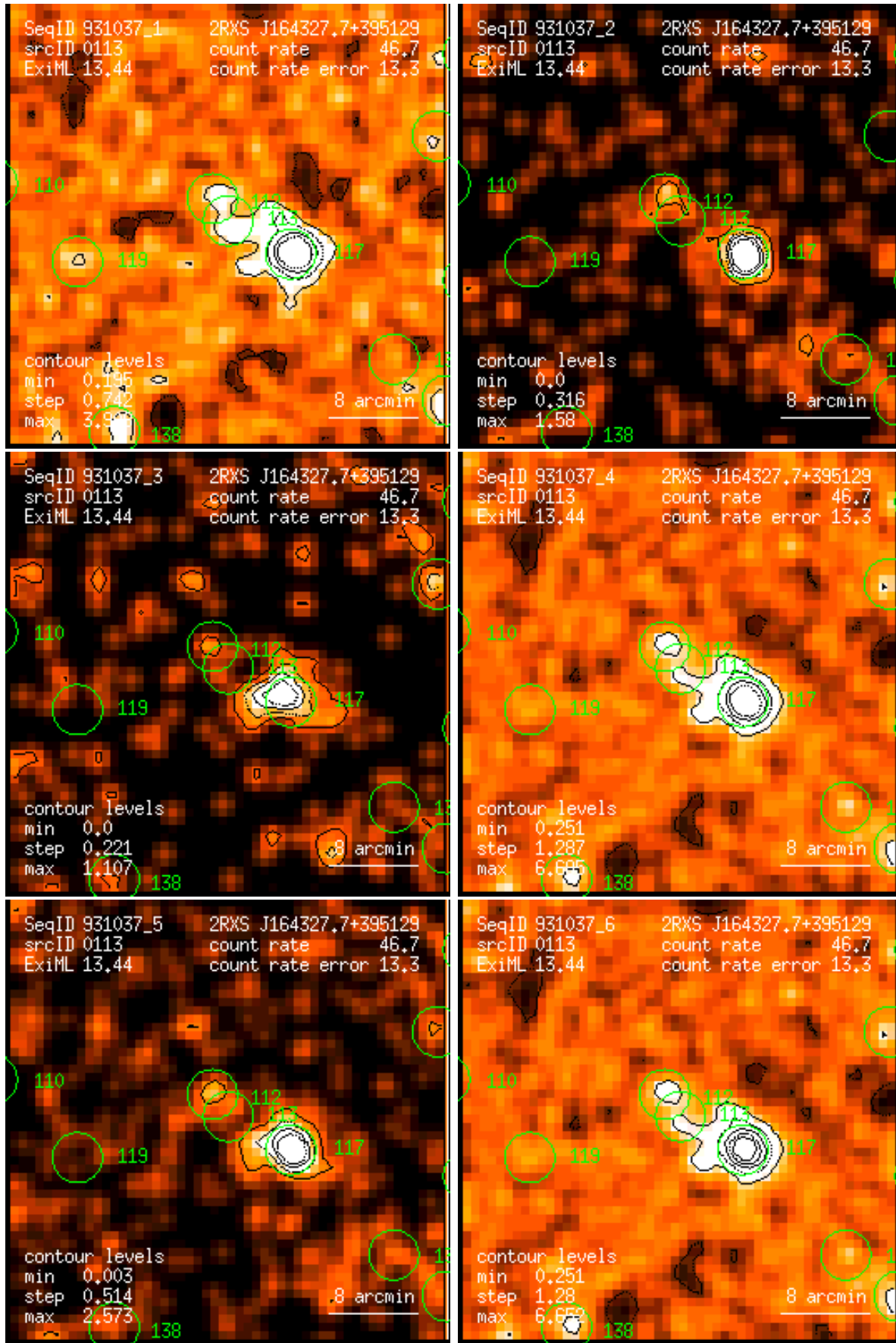
Figure 113: RASS 931037: detection 0113: band rate images, Gaussian filter: (1) PSPC channels 11 – 41, (2) 52 – 90, (3) 91 – 201, (4) 11 – 235, (5) 52 – 201, (6) 11 – 201. Broad band rates in counts/ks. Band rate contour levels in counts/ks/arcmin 2 .
