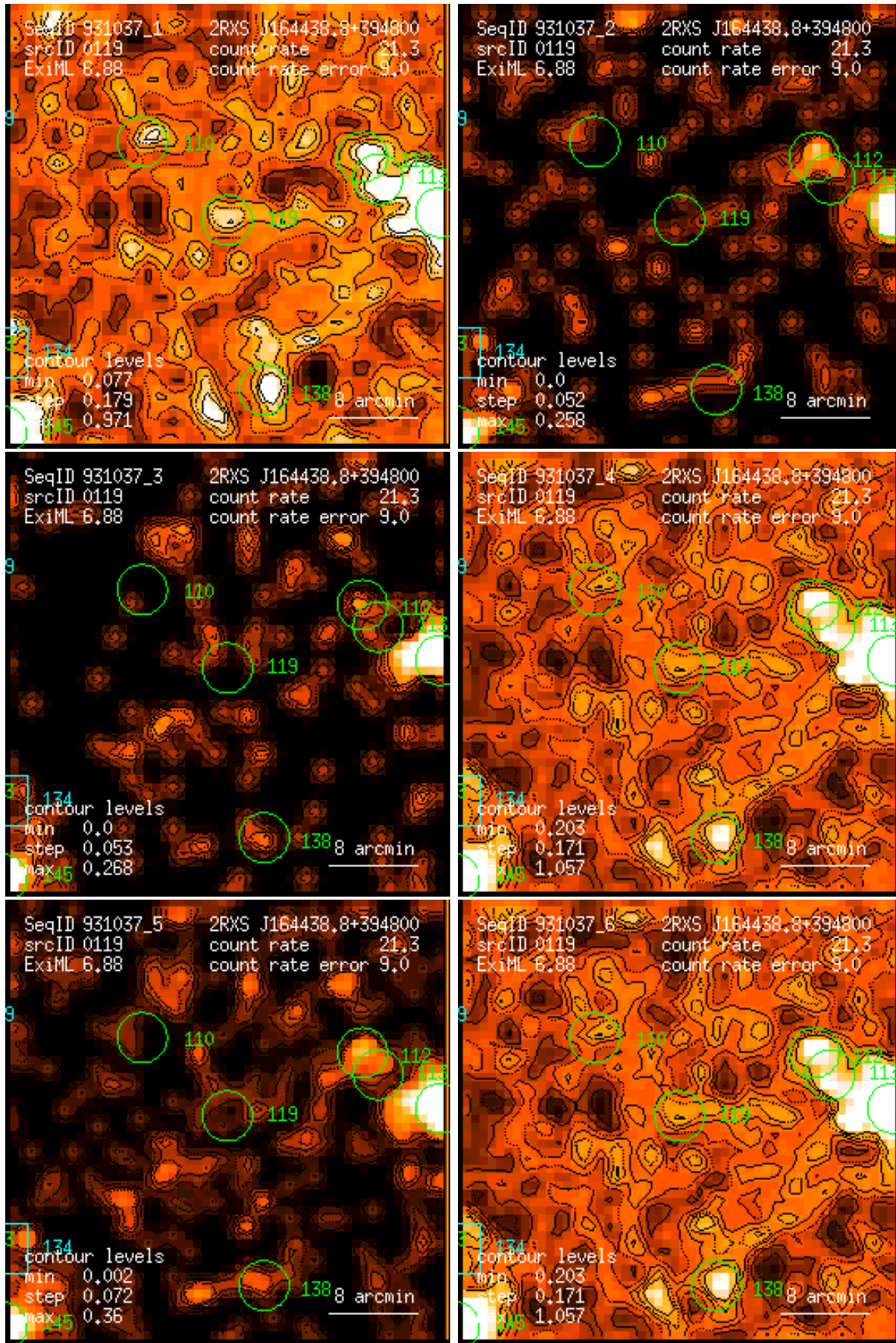
Figure 119: RASS 931037: detection 0119: band rate images, Gaussian filter: (1) PSPC channels 11 – 41, (2) 52 – 90, (3) 91 – 201, (4) 11 – 235, (5) 52 – 201, (6) 11 – 201. Broad band rates in counts/ks. Band rate contour levels in counts/ks/arcmin 2 .
