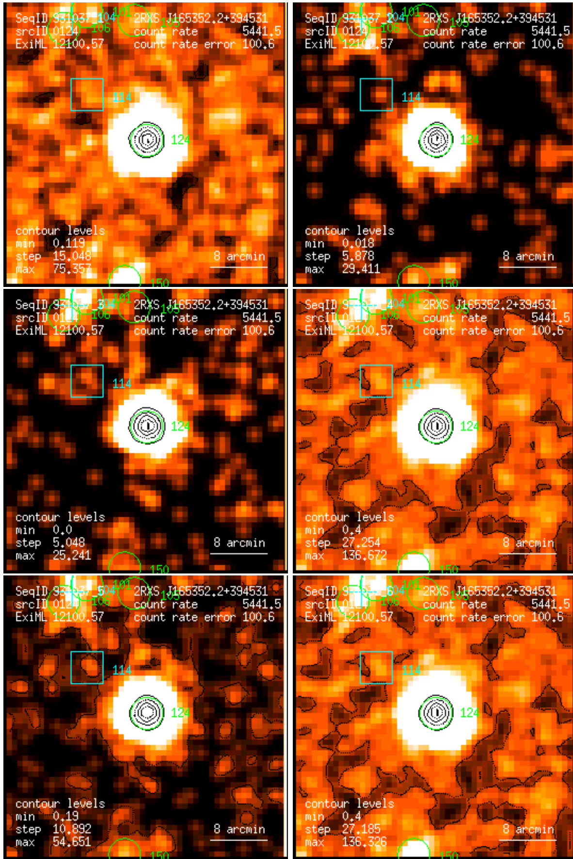
Figure 124: RASS 931037: detection 0124: band rate images, Gaussian filter: (1) PSPC channels 11 – 41, (2) 52 – 90, (3) 91 – 201, (4) 11 – 235, (5) 52 – 201, (6) 11 – 201. Broad band rates in counts/ks. Band rate contour levels in counts/ks/arcmin 2 .
