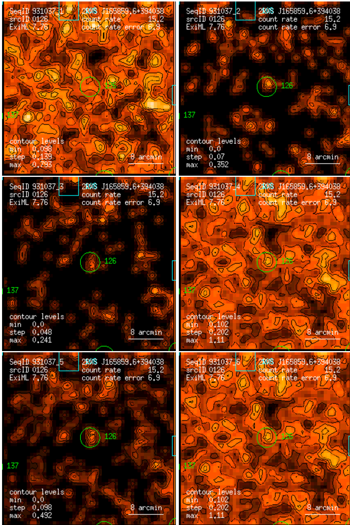
Figure 126: RASS 931037: detection 0126: band rate images, Gaussian filter: (1) PSPC channels 11 – 41, (2) 52 – 90, (3) 91 – 201, (4) 11 – 235, (5) 52 – 201, (6) 11 – 201. Broad band rates in counts/ks. Band rate contour levels in counts/ks/arcmin 2 .
