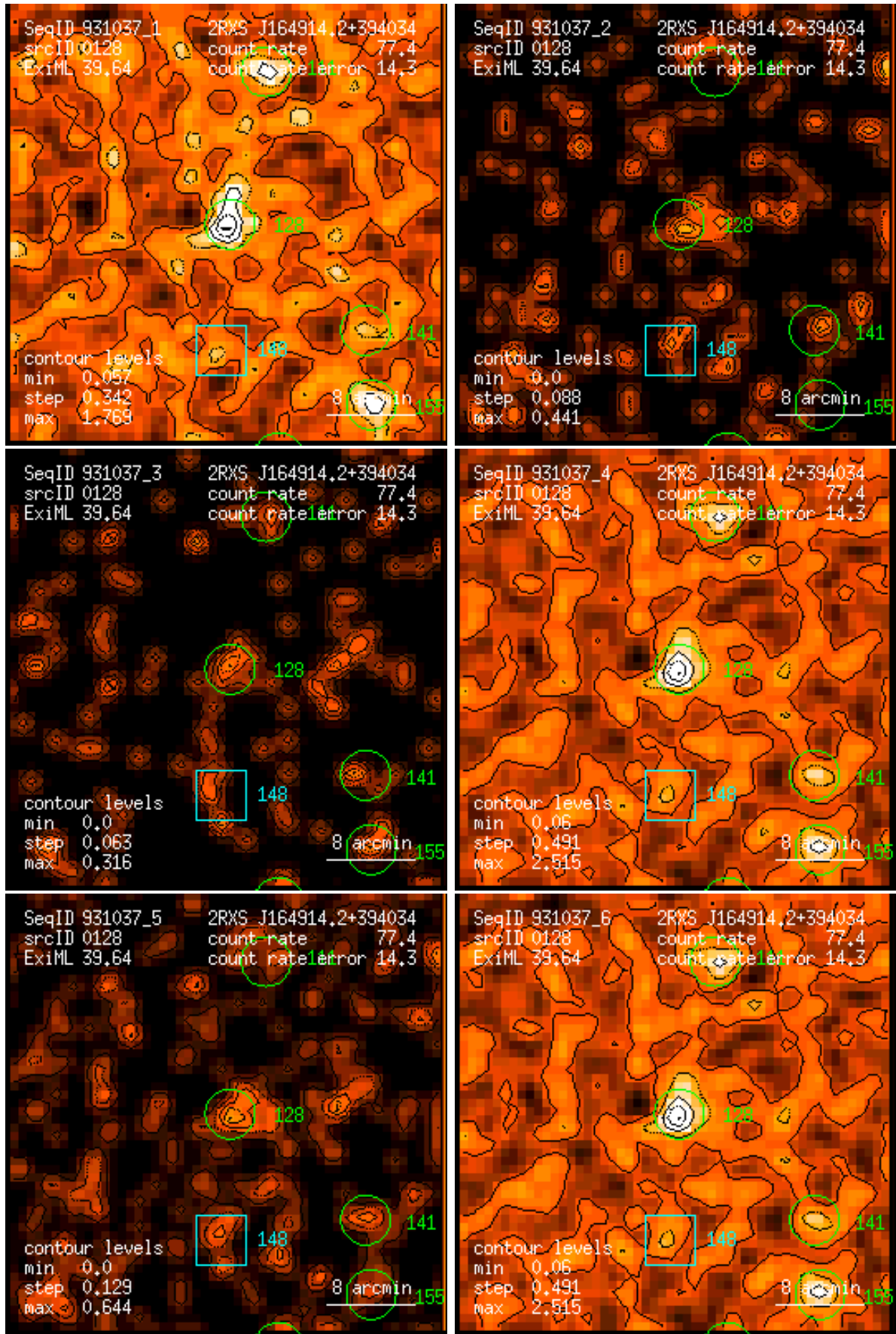
Figure 128: RASS 931037: detection 0128: band rate images, Gaussian filter: (1) PSPC channels 11 – 41, (2) 52 – 90, (3) 91 – 201, (4) 11 – 235, (5) 52 – 201, (6) 11 – 201. Broad band rates in counts/ks. Band rate contour levels in counts/ks/arcmin 2 .
