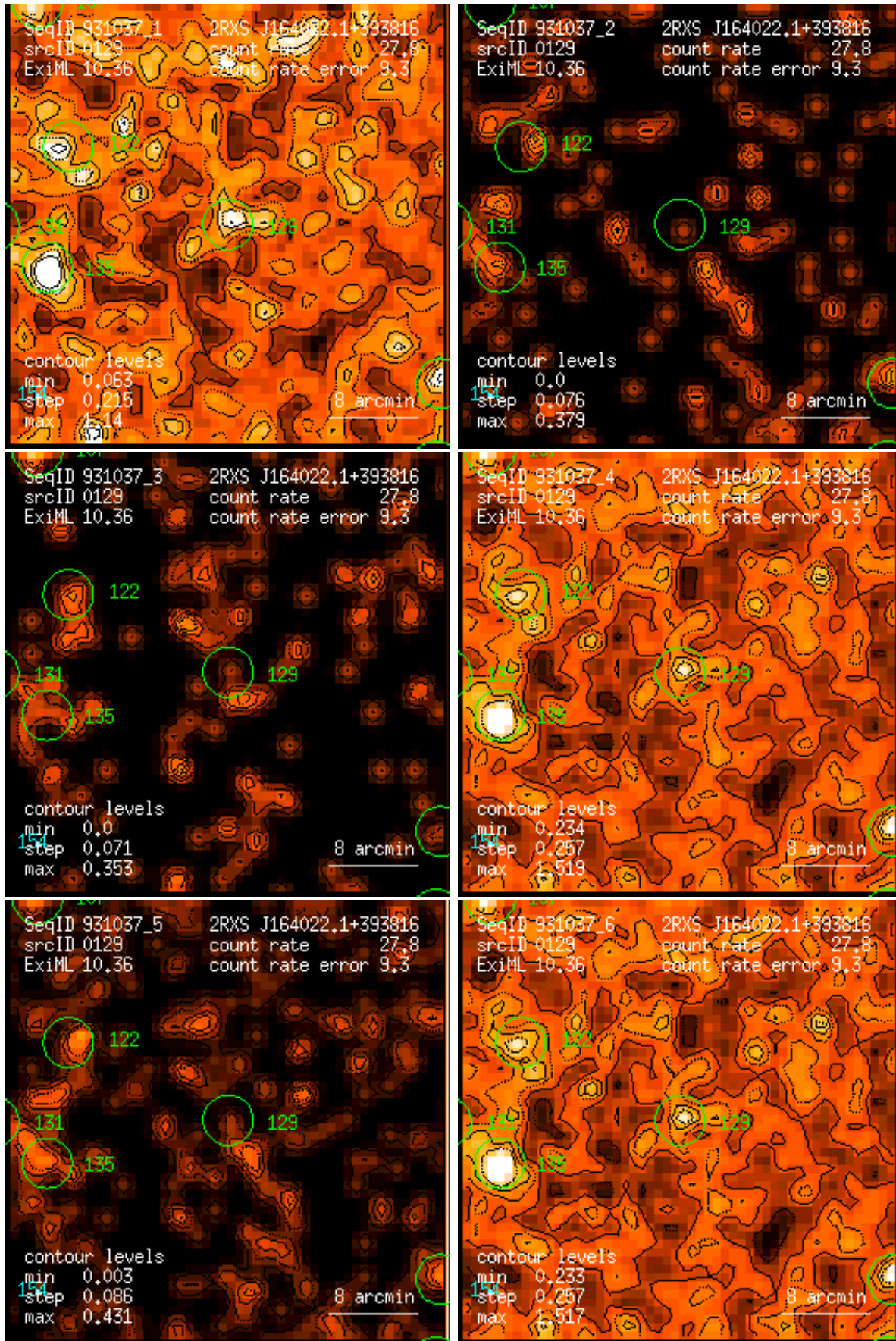
Figure 129: RASS 931037: detection 0129: band rate images, Gaussian filter: (1) PSPC channels 11 – 41, (2) 52 – 90, (3) 91 – 201, (4) 11 – 235, (5) 52 – 201, (6) 11 – 201. Broad band rates in counts/ks. Band rate contour levels in counts/ks/arcmin 2 .
