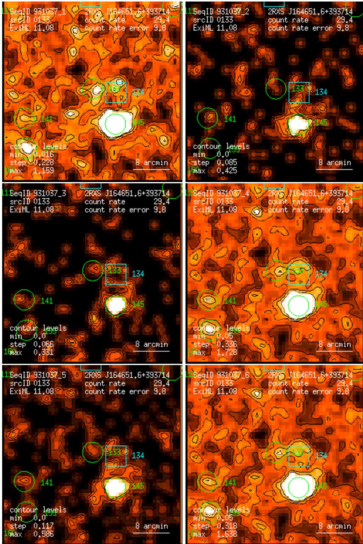
Figure 133: RASS 931037: detection 0133: band rate images, Gaussian filter: (1) PSPC channels 11 – 41, (2) 52 – 90, (3) 91 – 201, (4) 11 – 235, (5) 52 – 201, (6) 11 – 201. Broad band rates in counts/ks. Band rate contour levels in counts/ks/arcmin 2 .
