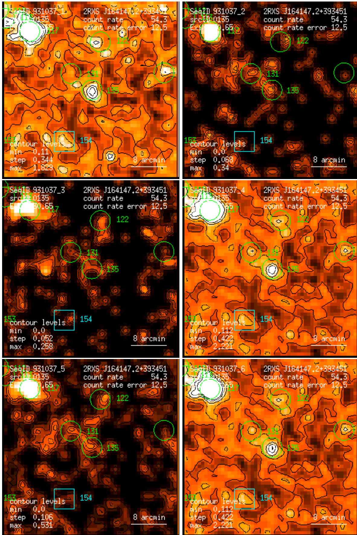
Figure 135: RASS 931037: detection 0135: band rate images, Gaussian filter: (1) PSPC channels 11 – 41, (2) 52 – 90, (3) 91 – 201, (4) 11 – 235, (5) 52 – 201, (6) 11 – 201. Broad band rates in counts/ks. Band rate contour levels in counts/ks/arcmin 2 .
