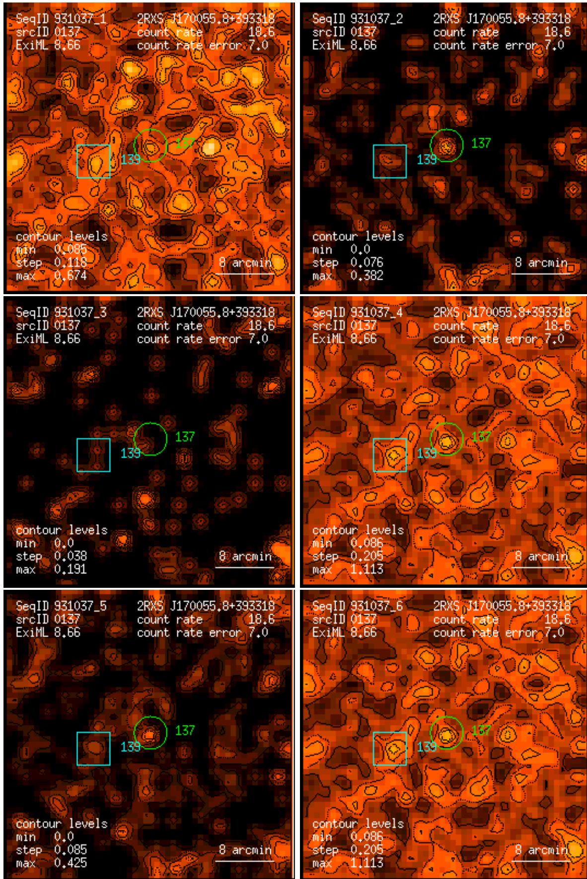
Figure 137: RASS 931037: detection 0137: band rate images, Gaussian filter: (1) PSPC channels 11 – 41, (2) 52 – 90, (3) 91 – 201, (4) 11 – 235, (5) 52 – 201, (6) 11 – 201. Broad band rates in counts/ks. Band rate contour levels in counts/ks/arcmin 2 .
