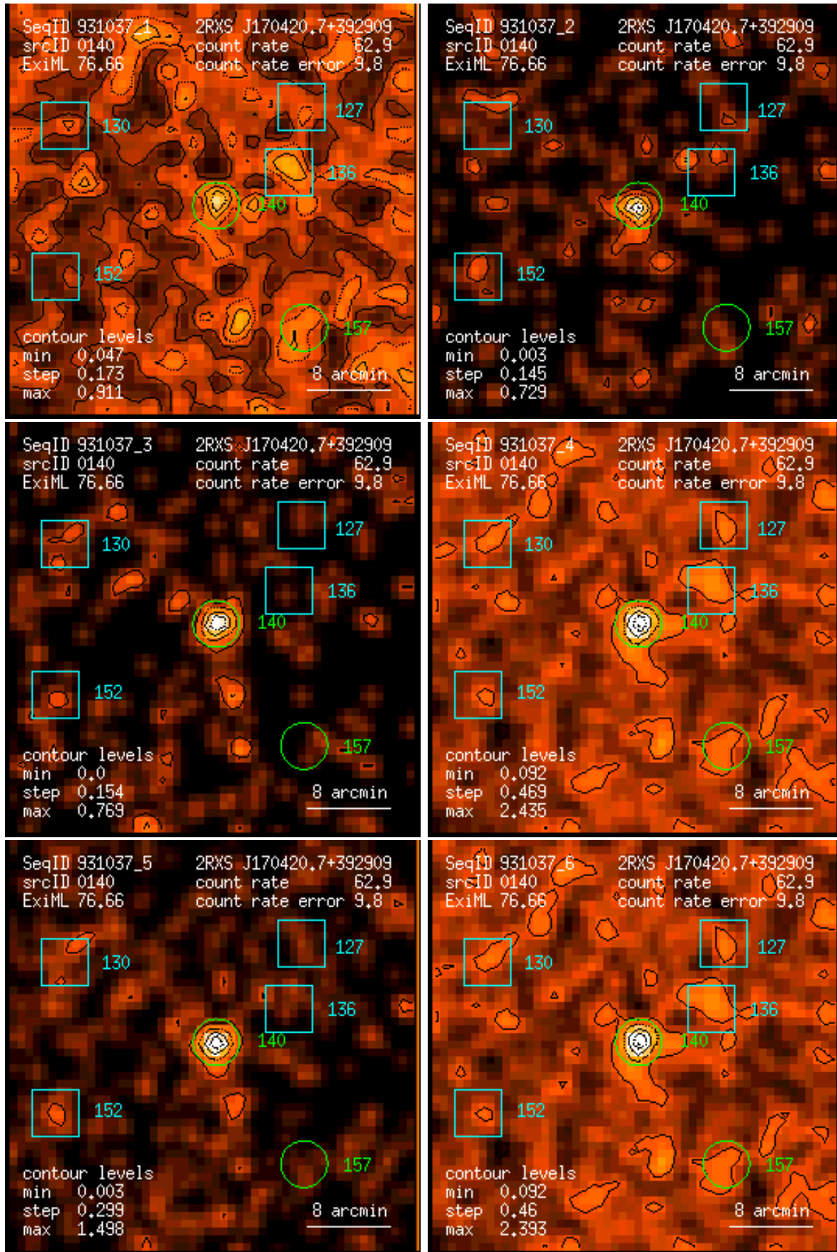
Figure 140: RASS 931037: detection 0140: band rate images, Gaussian filter: (1) PSPC channels 11 – 41, (2) 52 – 90, (3) 91 – 201, (4) 11 – 235, (5) 52 – 201, (6) 11 – 201. Broad band rates in counts/ks. Band rate contour levels in counts/ks/arcmin 2 .
