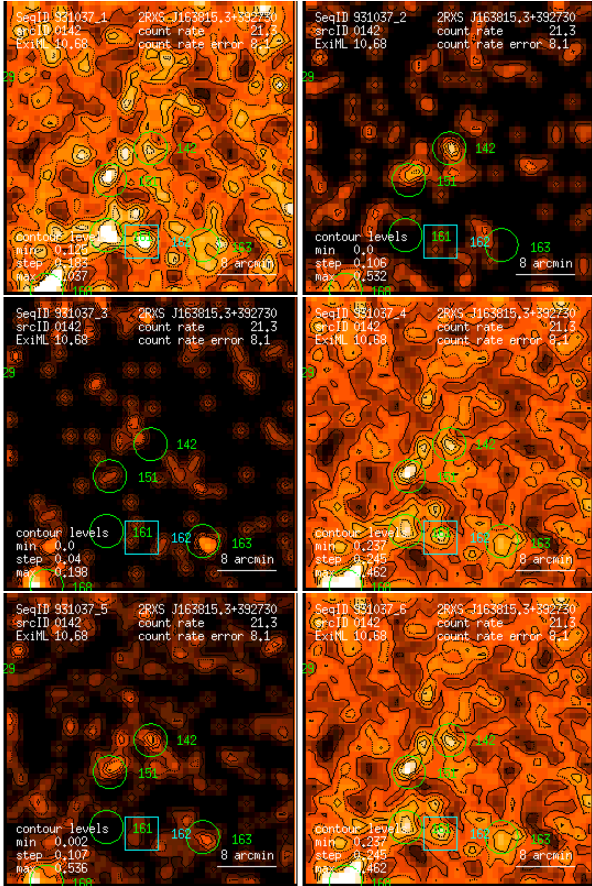
Figure 142: RASS 931037: detection 0142: band rate images, Gaussian filter: (1) PSPC channels 11 – 41, (2) 52 – 90, (3) 91 – 201, (4) 11 – 235, (5) 52 – 201, (6) 11 – 201. Broad band rates in counts/ks. Band rate contour levels in counts/ks/arcmin 2 .
