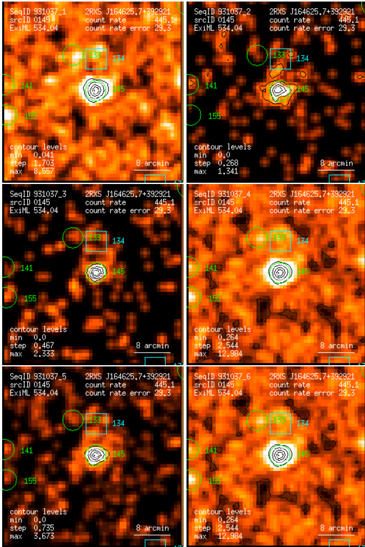
Figure 145: RASS 931037: detection 0145: band rate images, Gaussian filter: (1) PSPC channels 11 – 41, (2) 52 – 90, (3) 91 – 201, (4) 11 – 235, (5) 52 – 201, (6) 11 – 201. Broad band rates in counts/ks. Band rate contour levels in counts/ks/arcmin 2 .
