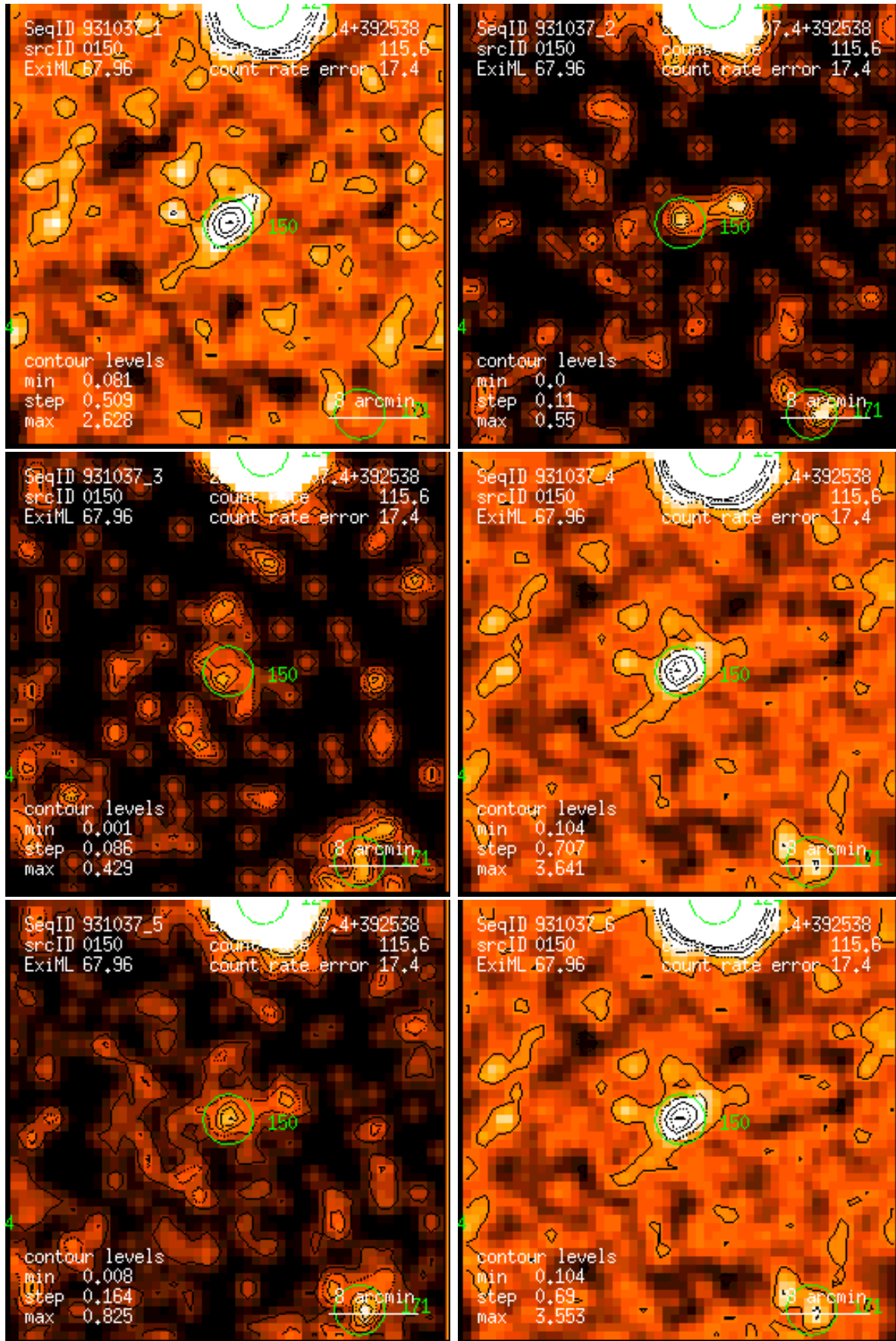
Figure 150: RASS 931037: detection 0150: band rate images, Gaussian filter: (1) PSPC channels 11 – 41, (2) 52 – 90, (3) 91 – 201, (4) 11 – 235, (5) 52 – 201, (6) 11 – 201. Broad band rates in counts/ks. Band rate contour levels in counts/ks/arcmin 2 .
