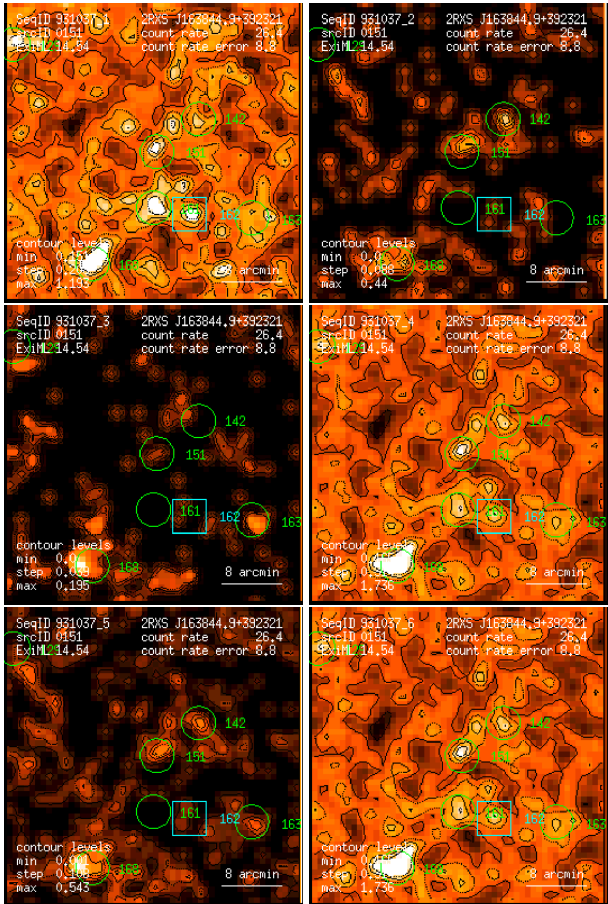
Figure 151: RASS 931037: detection 0151: band rate images, Gaussian filter: (1) PSPC channels 11 – 41, (2) 52 – 90, (3) 91 – 201, (4) 11 – 235, (5) 52 – 201, (6) 11 – 201. Broad band rates in counts/ks. Band rate contour levels in counts/ks/arcmin 2 .
