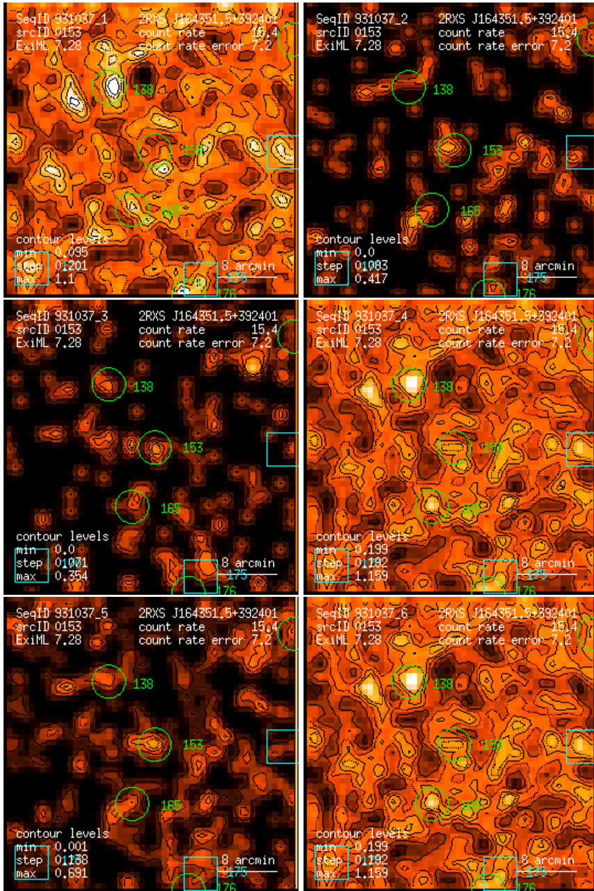
Figure 153: RASS 931037: detection 0153: band rate images, Gaussian filter: (1) PSPC channels 11 – 41, (2) 52 – 90, (3) 91 – 201, (4) 11 – 235, (5) 52 – 201, (6) 11 – 201. Broad band rates in counts/ks. Band rate contour levels in counts/ks/arcmin 2 .
