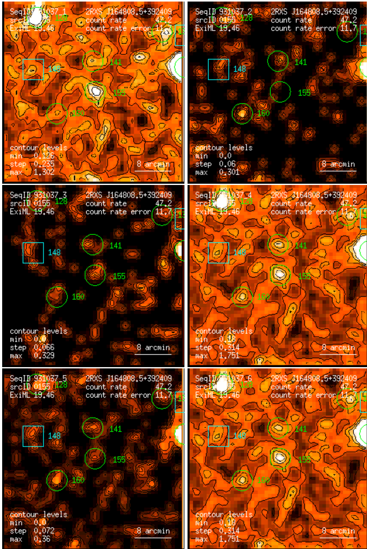
Figure 155: RASS 931037: detection 0155: band rate images, Gaussian filter: (1) PSPC channels 11 – 41, (2) 52 – 90, (3) 91 – 201, (4) 11 – 235, (5) 52 – 201, (6) 11 – 201. Broad band rates in counts/ks. Band rate contour levels in counts/ks/arcmin 2 .
