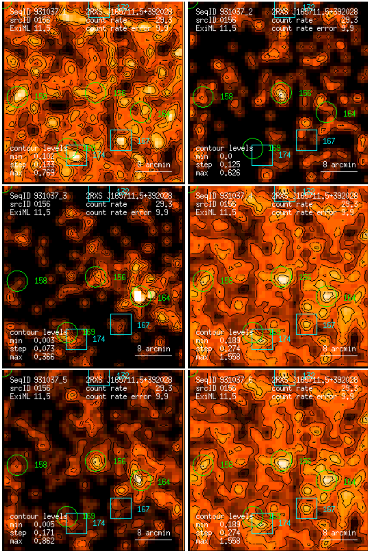
Figure 156: RASS 931037: detection 0156: band rate images, Gaussian filter: (1) PSPC channels 11 – 41, (2) 52 – 90, (3) 91 – 201, (4) 11 – 235, (5) 52 – 201, (6) 11 – 201. Broad band rates in counts/ks. Band rate contour levels in counts/ks/arcmin 2 .
