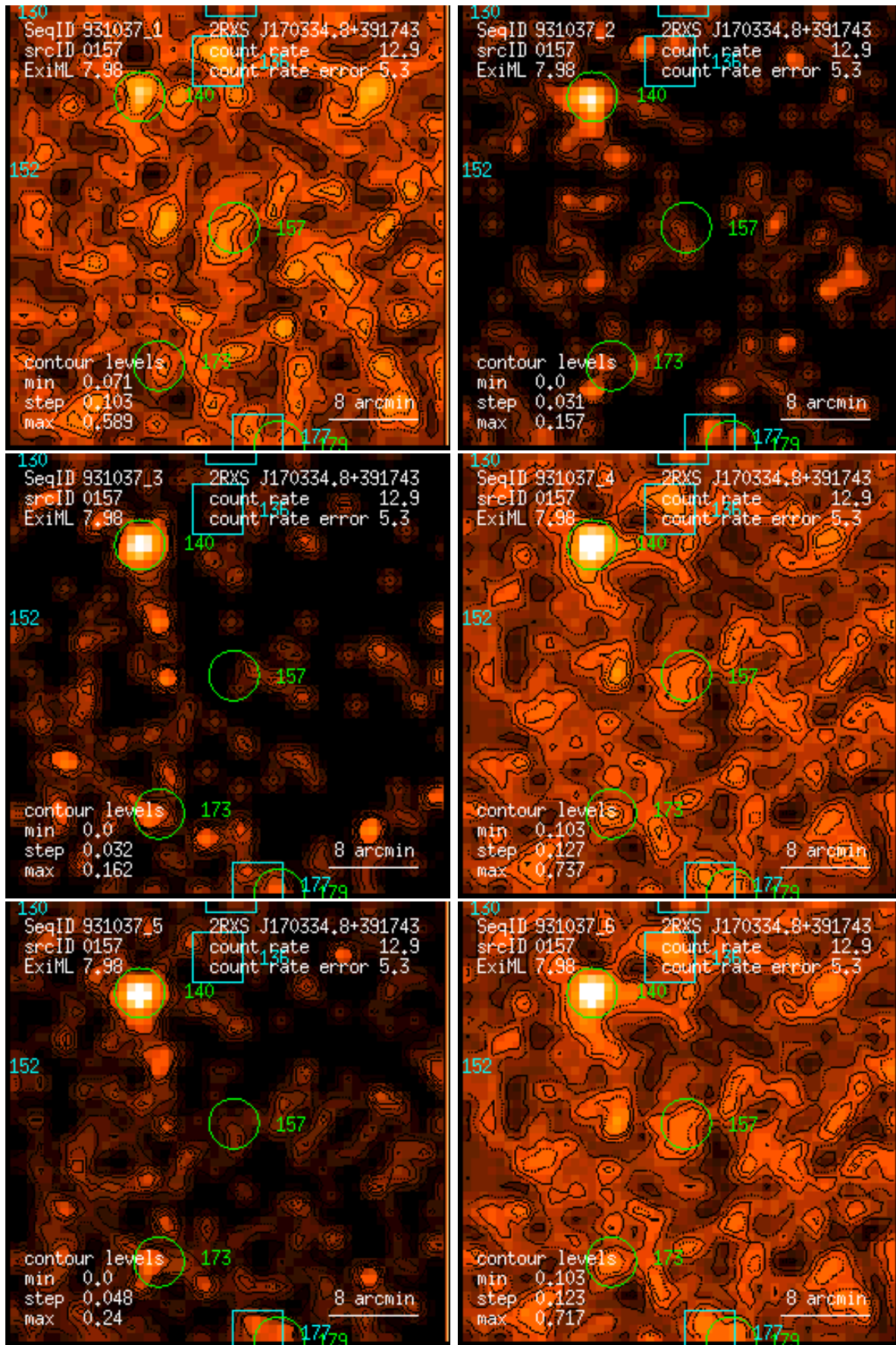
Figure 157: RASS 931037: detection 0157: band rate images, Gaussian filter: (1) PSPC channels 11 – 41, (2) 52 – 90, (3) 91 – 201, (4) 11 – 235, (5) 52 – 201, (6) 11 – 201. Broad band rates in counts/ks. Band rate contour levels in counts/ks/arcmin 2 .
