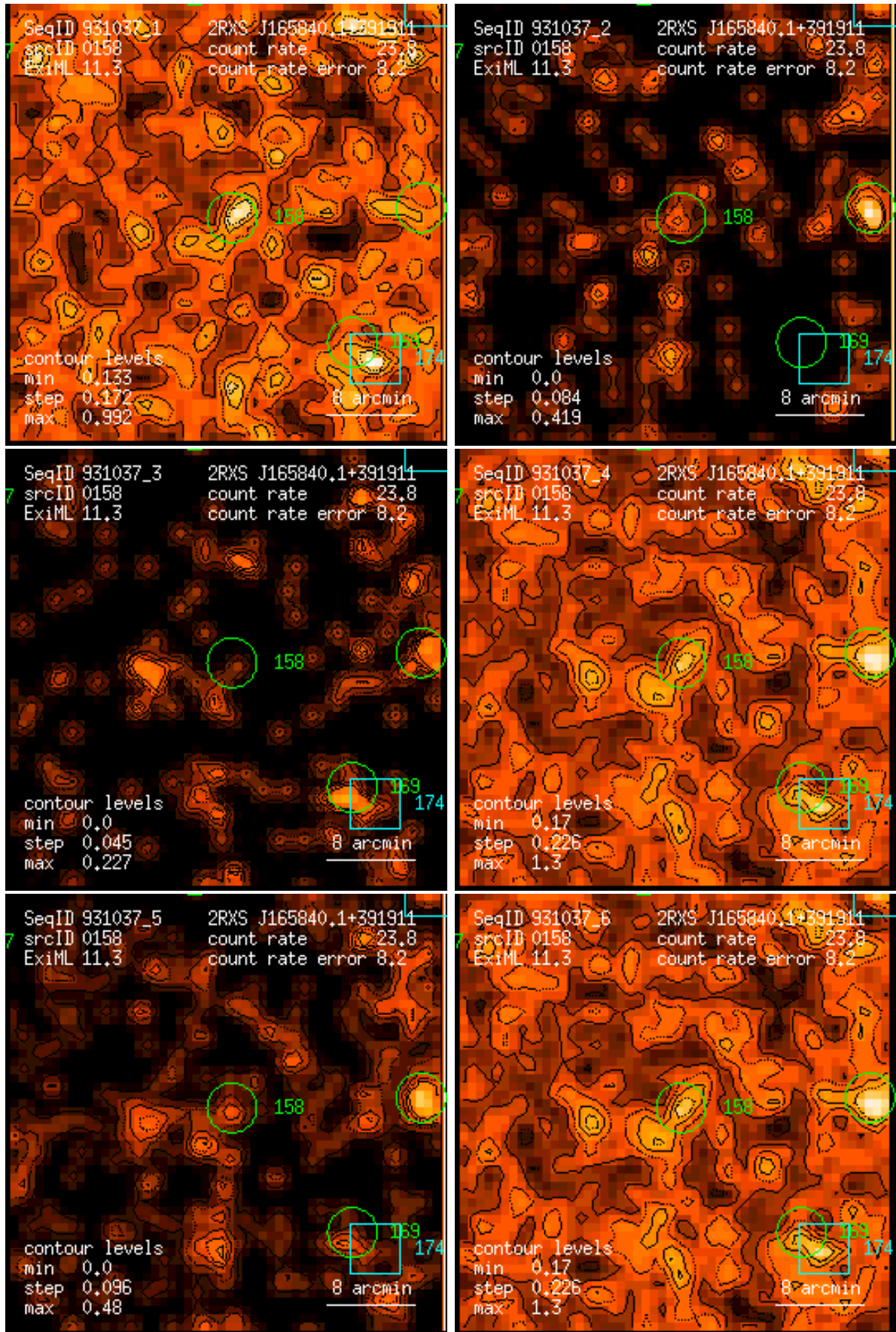
Figure 158: RASS 931037: detection 0158: band rate images, Gaussian filter: (1) PSPC channels 11 – 41, (2) 52 – 90, (3) 91 – 201, (4) 11 – 235, (5) 52 – 201, (6) 11 – 201. Broad band rates in counts/ks. Band rate contour levels in counts/ks/arcmin 2 .
