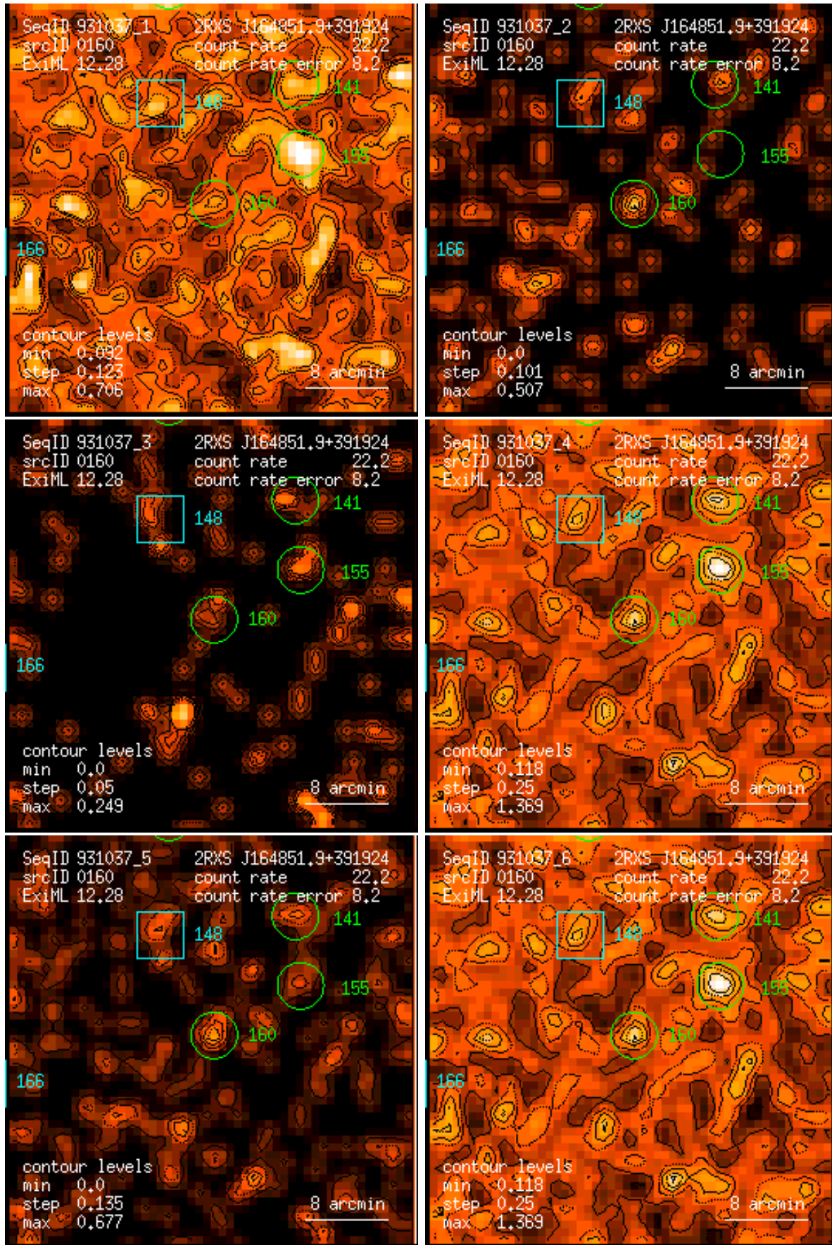
Figure 160: RASS 931037: detection 0160: band rate images, Gaussian filter: (1) PSPC channels 11 – 41, (2) 52 – 90, (3) 91 – 201, (4) 11 – 235, (5) 52 – 201, (6) 11 – 201. Broad band rates in counts/ks. Band rate contour levels in counts/ks/arcmin 2 .
