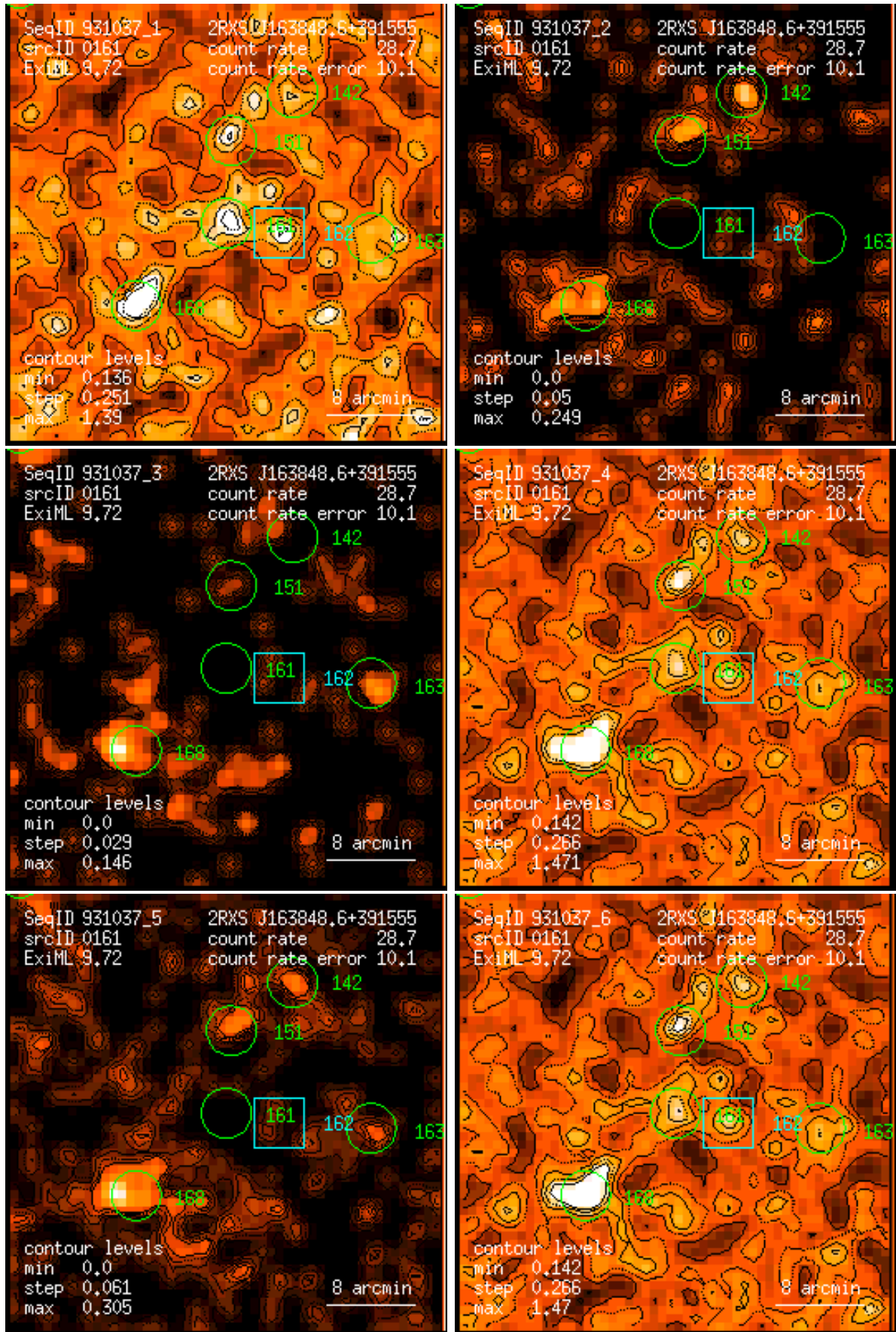
Figure 161: RASS 931037: detection 0161: band rate images, Gaussian filter: (1) PSPC channels 11 – 41, (2) 52 – 90, (3) 91 – 201, (4) 11 – 235, (5) 52 – 201, (6) 11 – 201. Broad band rates in counts/ks. Band rate contour levels in counts/ks/arcmin 2 .
