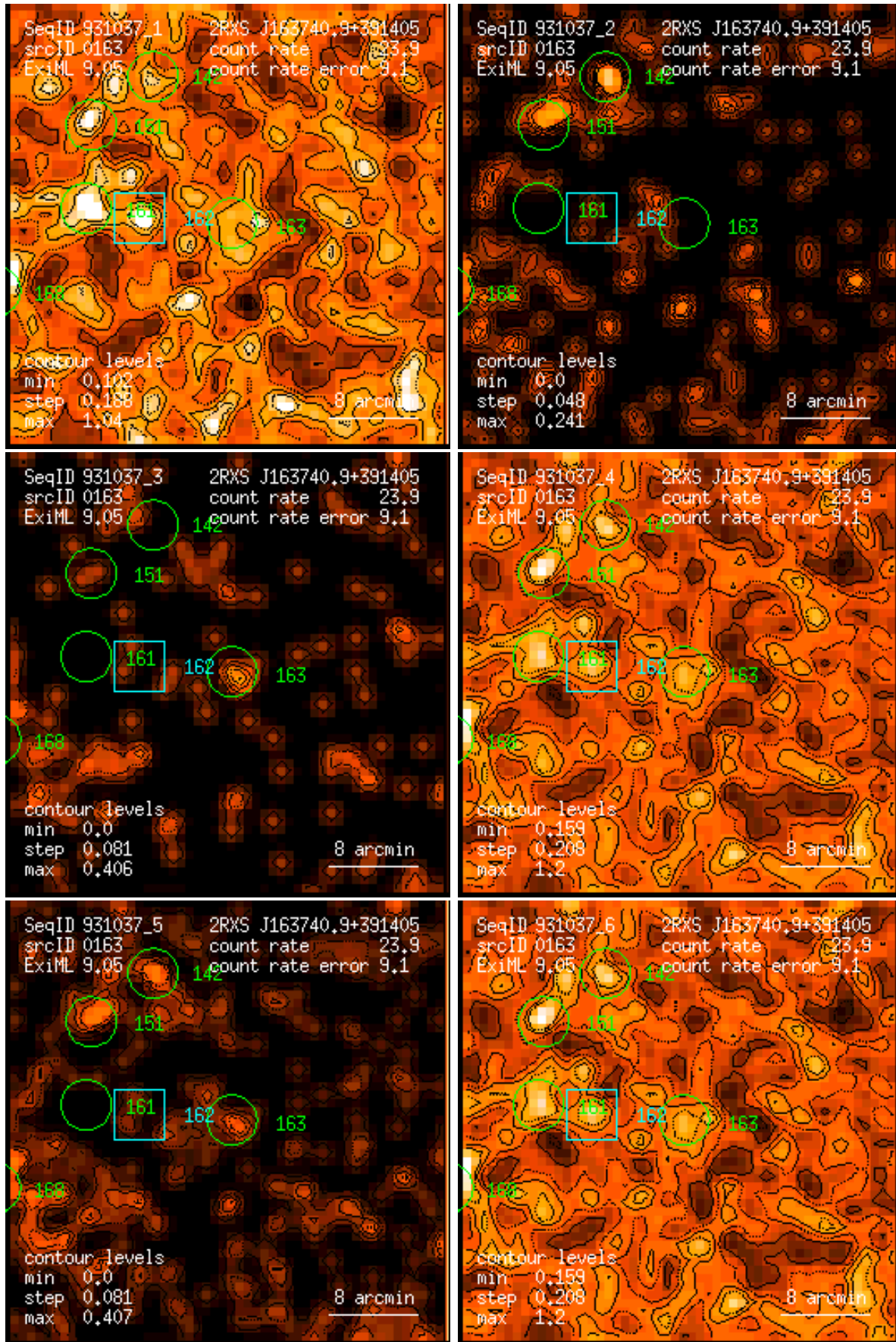
Figure 163: RASS 931037: detection 0163: band rate images, Gaussian filter: (1) PSPC channels 11 – 41, (2) 52 – 90, (3) 91 – 201, (4) 11 – 235, (5) 52 – 201, (6) 11 – 201. Broad band rates in counts/ks. Band rate contour levels in counts/ks/arcmin 2 .
