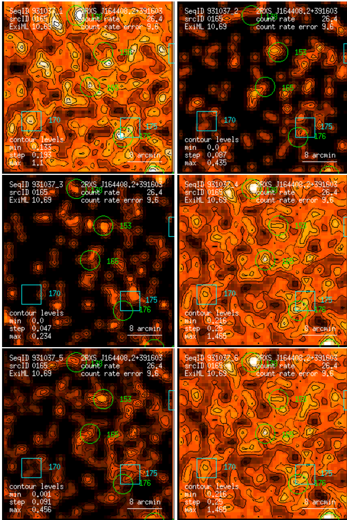
Figure 165: RASS 931037: detection 0165: band rate images, Gaussian filter: (1) PSPC channels 11 – 41, (2) 52 – 90, (3) 91 – 201, (4) 11 – 235, (5) 52 – 201, (6) 11 – 201. Broad band rates in counts/ks. Band rate contour levels in counts/ks/arcmin 2 .
