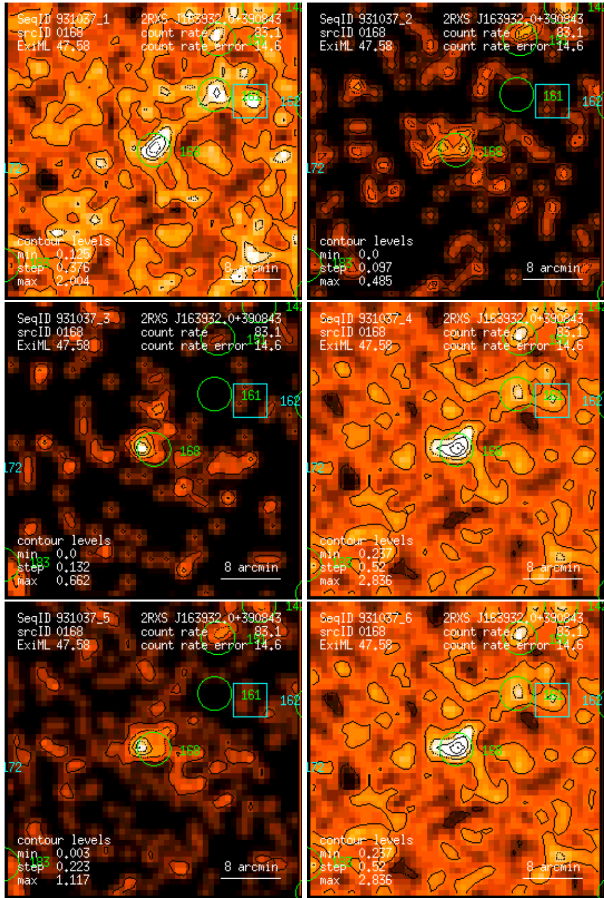
Figure 168: RASS 931037: detection 0168: band rate images, Gaussian filter: (1) PSPC channels 11 – 41, (2) 52 – 90, (3) 91 – 201, (4) 11 – 235, (5) 52 – 201, (6) 11 – 201. Broad band rates in counts/ks. Band rate contour levels in counts/ks/arcmin 2 .
