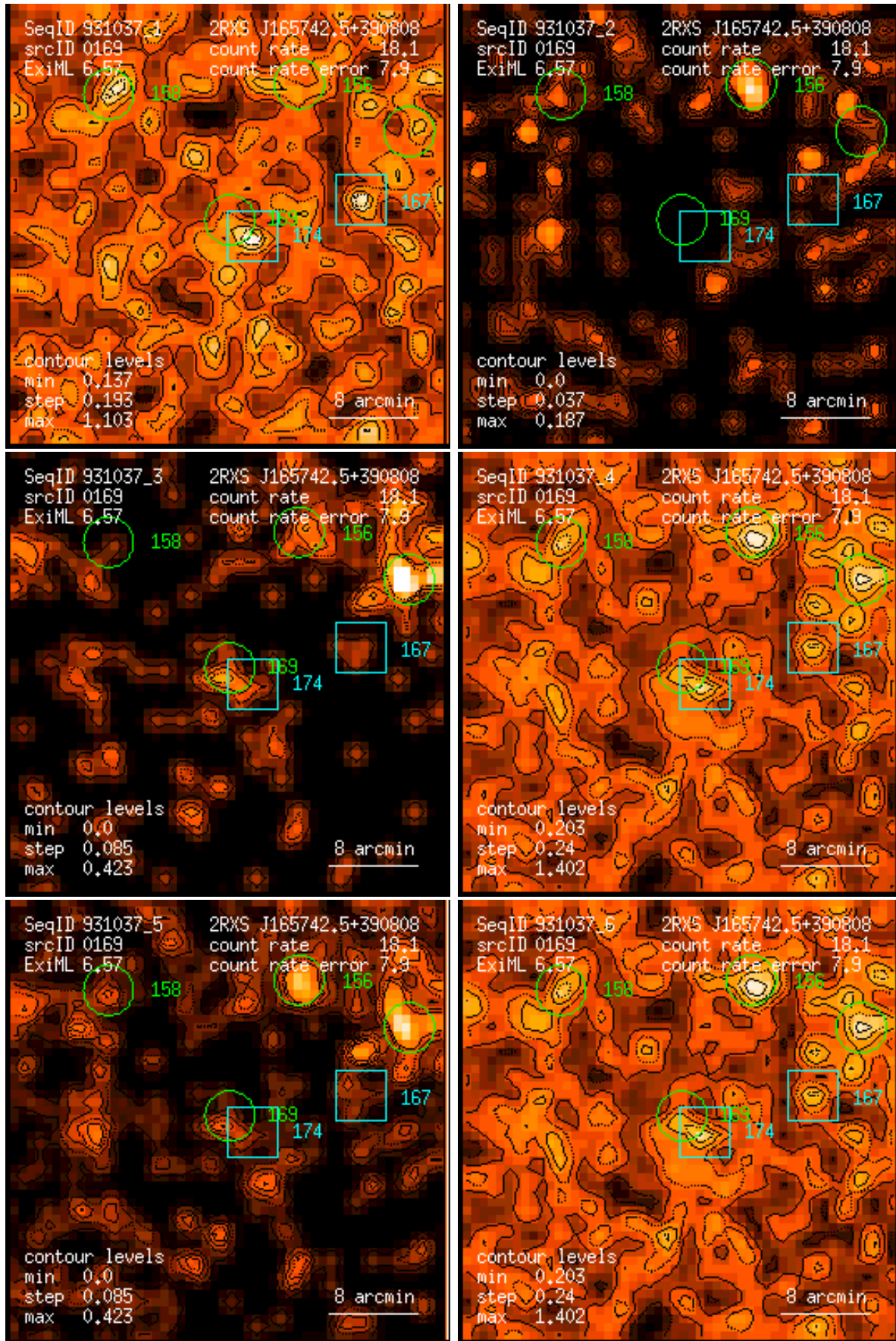
Figure 169: RASS 931037: detection 0169: band rate images, Gaussian filter: (1) PSPC channels 11 – 41, (2) 52 – 90, (3) 91 – 201, (4) 11 – 235, (5) 52 – 201, (6) 11 – 201. Broad band rates in counts/ks. Band rate contour levels in counts/ks/arcmin 2 .
