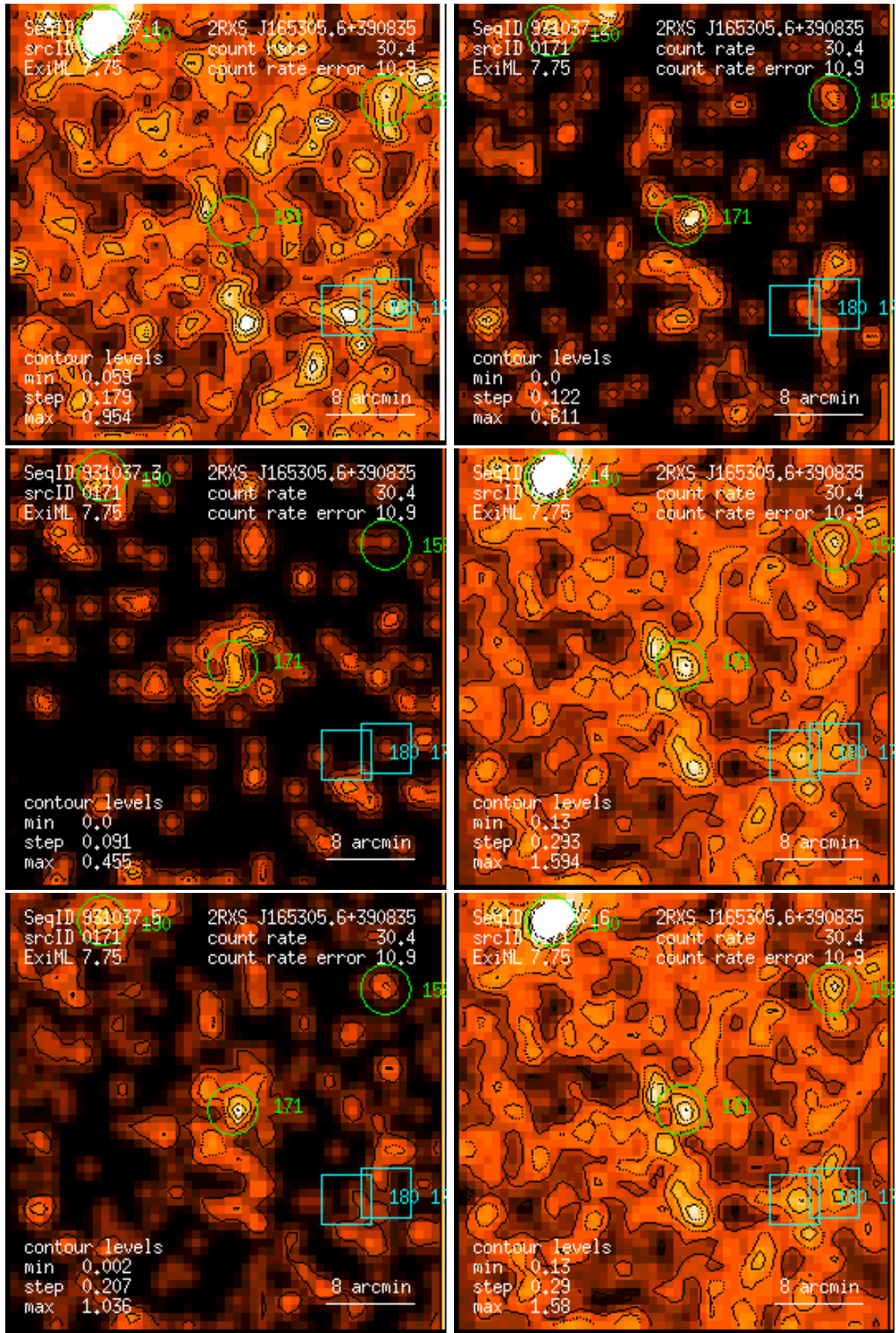
Figure 171: RASS 931037: detection 0171: band rate images, Gaussian filter: (1) PSPC channels 11 – 41, (2) 52 – 90, (3) 91 – 201, (4) 11 – 235, (5) 52 – 201, (6) 11 – 201. Broad band rates in counts/ks. Band rate contour levels in counts/ks/arcmin 2 .
