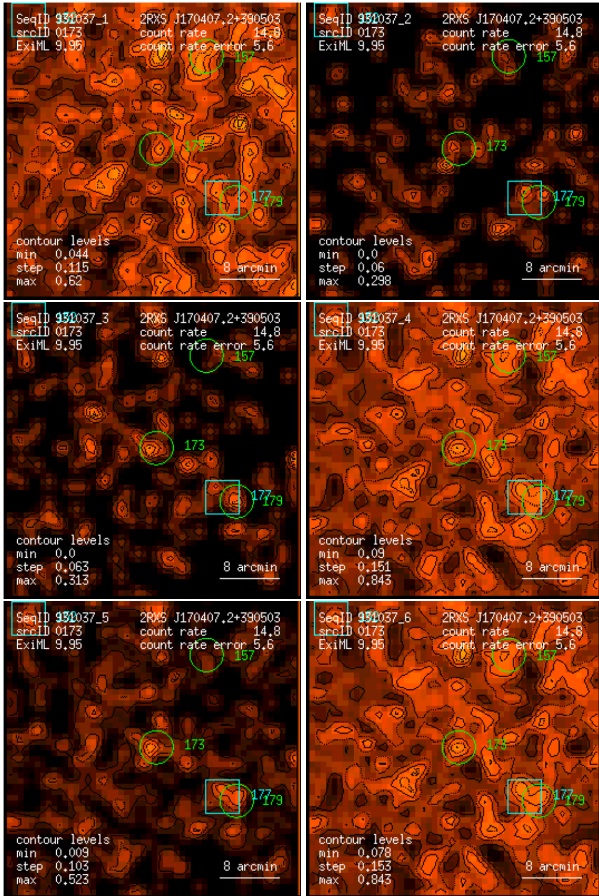
Figure 173: RASS 931037: detection 0173: band rate images, Gaussian filter: (1) PSPC channels 11 – 41, (2) 52 – 90, (3) 91 – 201, (4) 11 – 235, (5) 52 – 201, (6) 11 – 201. Broad band rates in counts/ks. Band rate contour levels in counts/ks/arcmin 2 .
