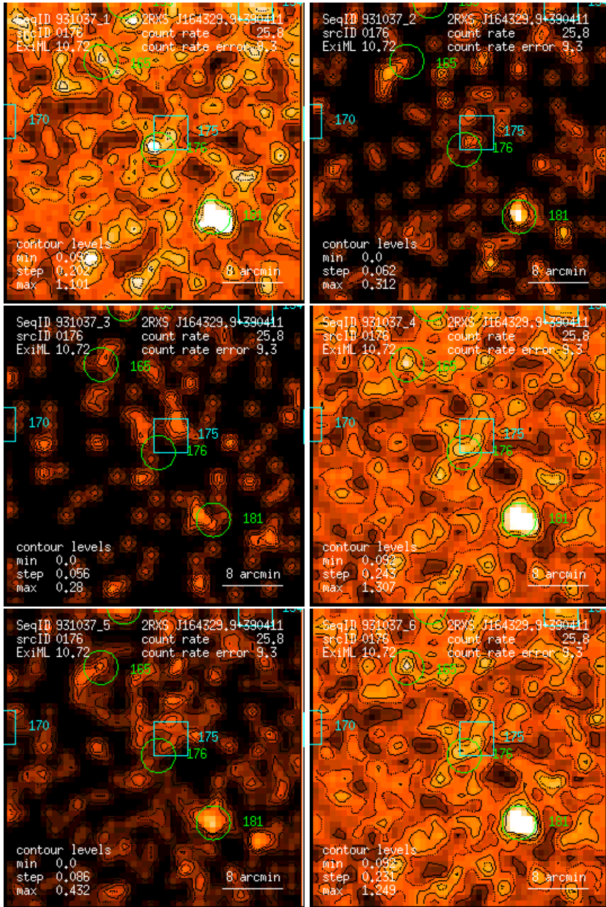
Figure 176: RASS 931037: detection 0176: band rate images, Gaussian filter: (1) PSPC channels 11 – 41, (2) 52 – 90, (3) 91 – 201, (4) 11 – 235, (5) 52 – 201, (6) 11 – 201. Broad band rates in counts/ks. Band rate contour levels in counts/ks/arcmin 2 .
