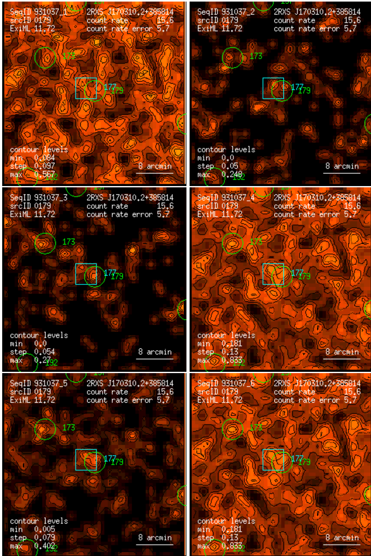
Figure 179: RASS 931037: detection 0179: band rate images, Gaussian filter: (1) PSPC channels 11 – 41, (2) 52 – 90, (3) 91 – 201, (4) 11 – 235, (5) 52 – 201, (6) 11 – 201. Broad band rates in counts/ks. Band rate contour levels in counts/ks/arcmin 2 .
