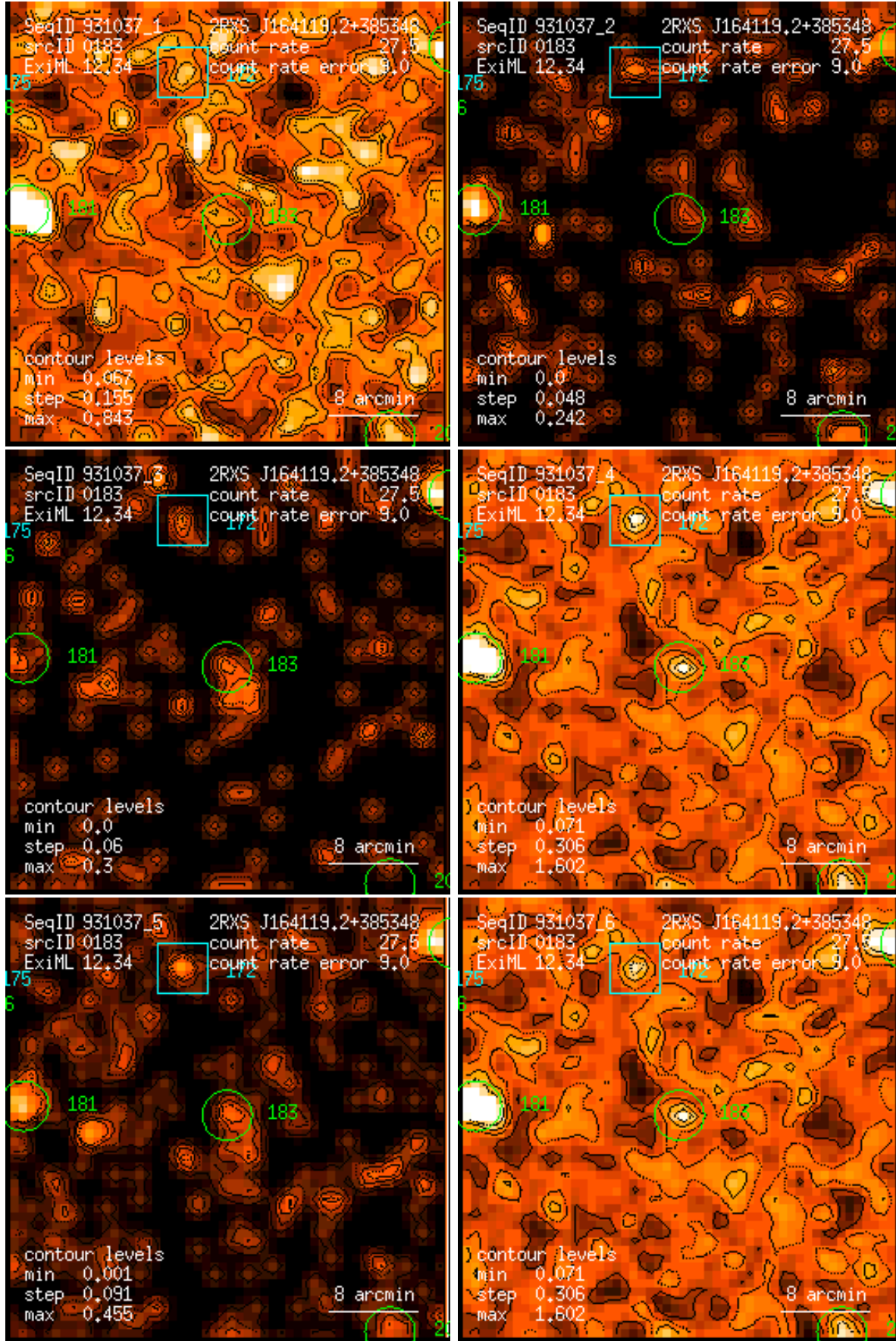
Figure 183: RASS 931037: detection 0183: band rate images, Gaussian filter: (1) PSPC channels 11 – 41, (2) 52 – 90, (3) 91 – 201, (4) 11 – 235, (5) 52 – 201, (6) 11 – 201. Broad band rates in counts/ks. Band rate contour levels in counts/ks/arcmin 2 .
