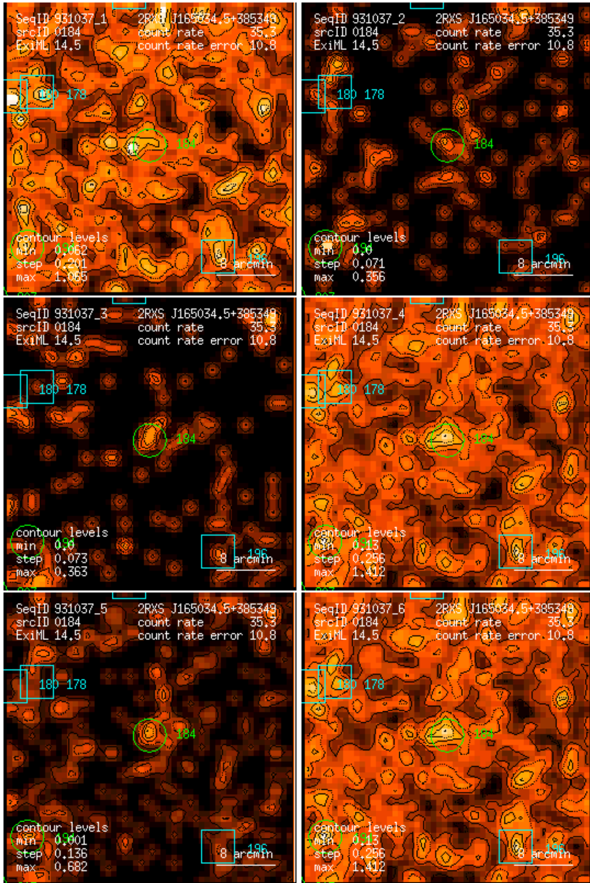
Figure 184: RASS 931037: detection 0184: band rate images, Gaussian filter: (1) PSPC channels 11 – 41, (2) 52 – 90, (3) 91 – 201, (4) 11 – 235, (5) 52 – 201, (6) 11 – 201. Broad band rates in counts/ks. Band rate contour levels in counts/ks/arcmin 2 .
