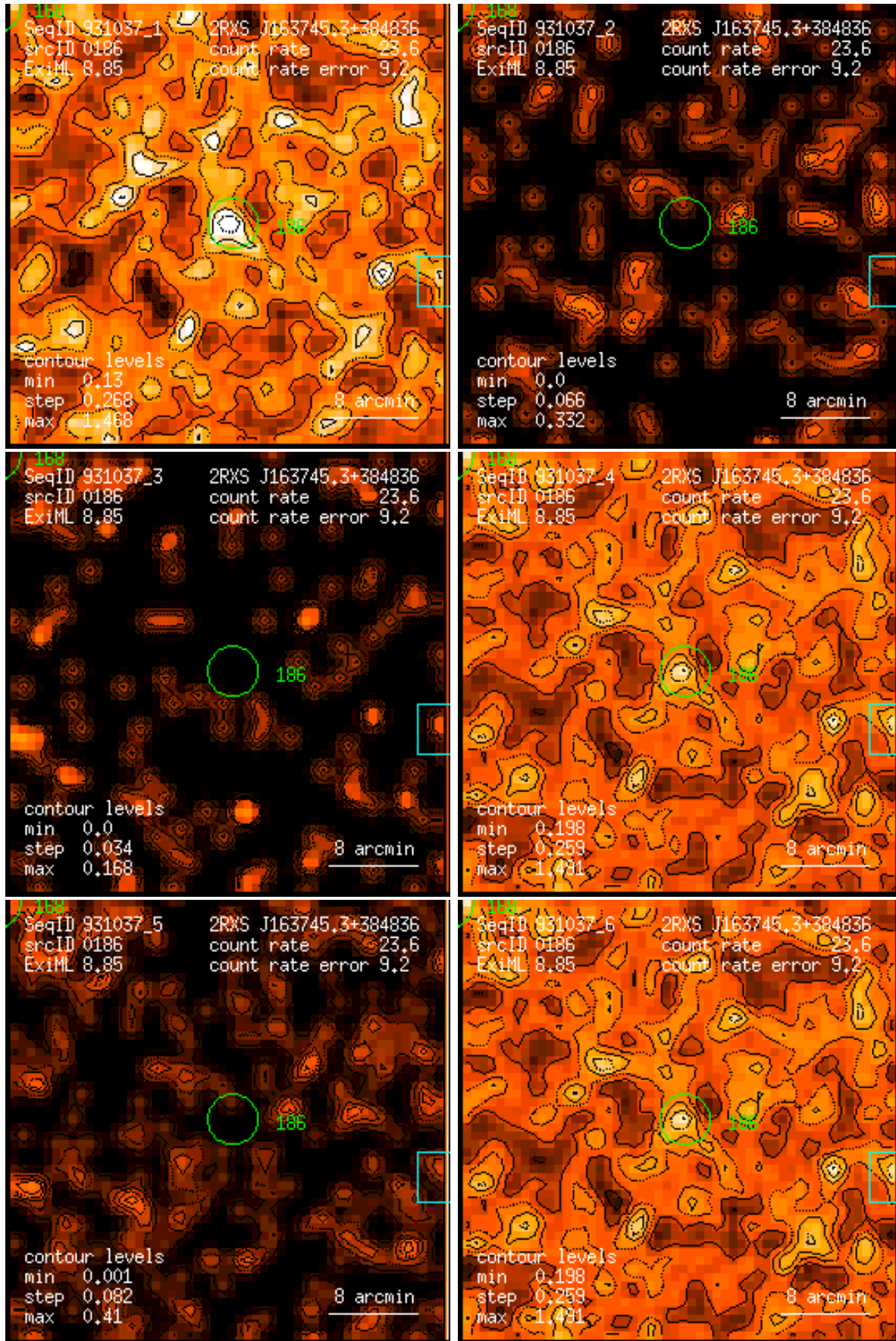
Figure 186: RASS 931037: detection 0186: band rate images, Gaussian filter: (1) PSPC channels 11 – 41, (2) 52 – 90, (3) 91 – 201, (4) 11 – 235, (5) 52 – 201, (6) 11 – 201. Broad band rates in counts/ks. Band rate contour levels in counts/ks/arcmin 2 .
