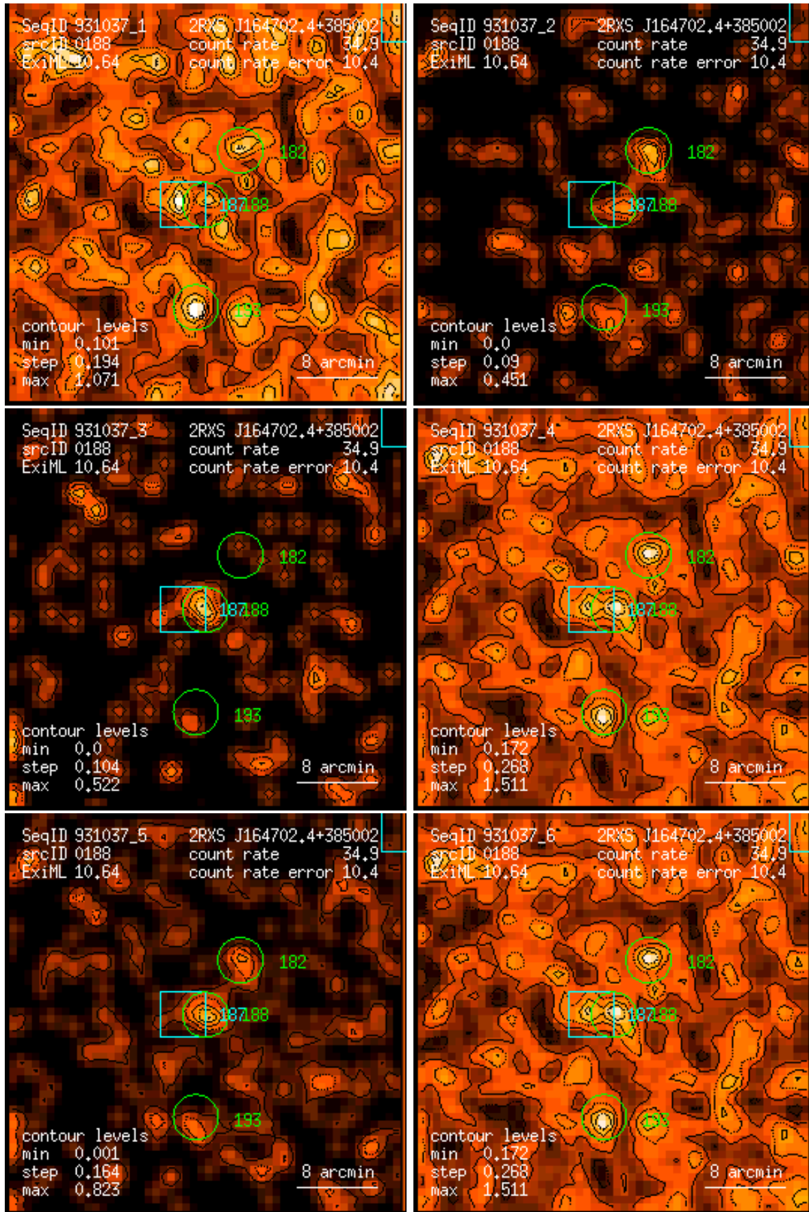
Figure 188: RASS 931037: detection 0188: band rate images, Gaussian filter: (1) PSPC channels 11 – 41, (2) 52 – 90, (3) 91 – 201, (4) 11 – 235, (5) 52 – 201, (6) 11 – 201. Broad band rates in counts/ks. Band rate contour levels in counts/ks/arcmin 2 .
