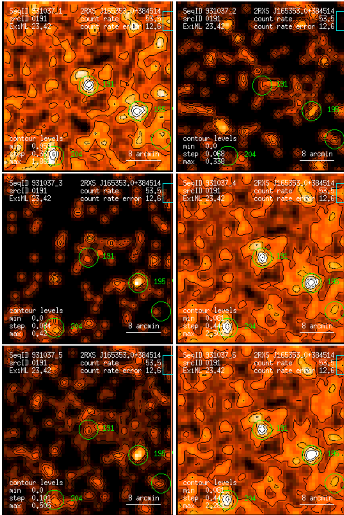
Figure 191: RASS 931037: detection 0191: band rate images, Gaussian filter: (1) PSPC channels 11 – 41, (2) 52 – 90, (3) 91 – 201, (4) 11 – 235, (5) 52 – 201, (6) 11 – 201. Broad band rates in counts/ks. Band rate contour levels in counts/ks/arcmin 2 .
