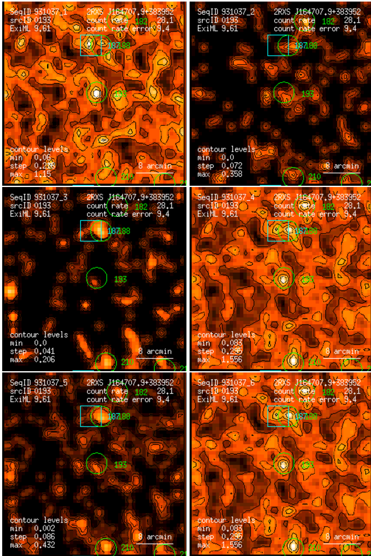
Figure 193: RASS 931037: detection 0193: band rate images, Gaussian filter: (1) PSPC channels 11 – 41, (2) 52 – 90, (3) 91 – 201, (4) 11 – 235, (5) 52 – 201, (6) 11 – 201. Broad band rates in counts/ks. Band rate contour levels in counts/ks/arcmin 2 .
