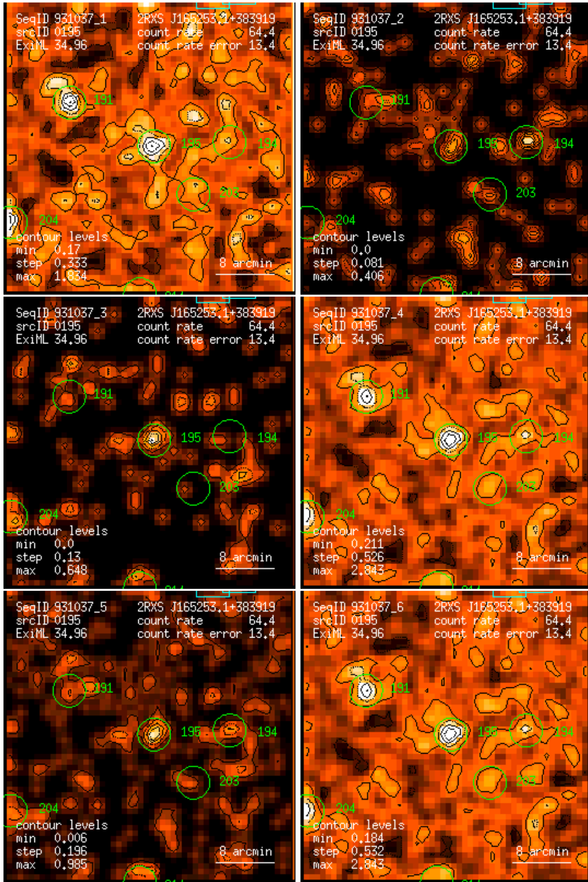
Figure 195: RASS 931037: detection 0195: band rate images, Gaussian filter: (1) PSPC channels 11 – 41, (2) 52 – 90, (3) 91 – 201, (4) 11 – 235, (5) 52 – 201, (6) 11 – 201. Broad band rates in counts/ks. Band rate contour levels in counts/ks/arcmin 2 .
