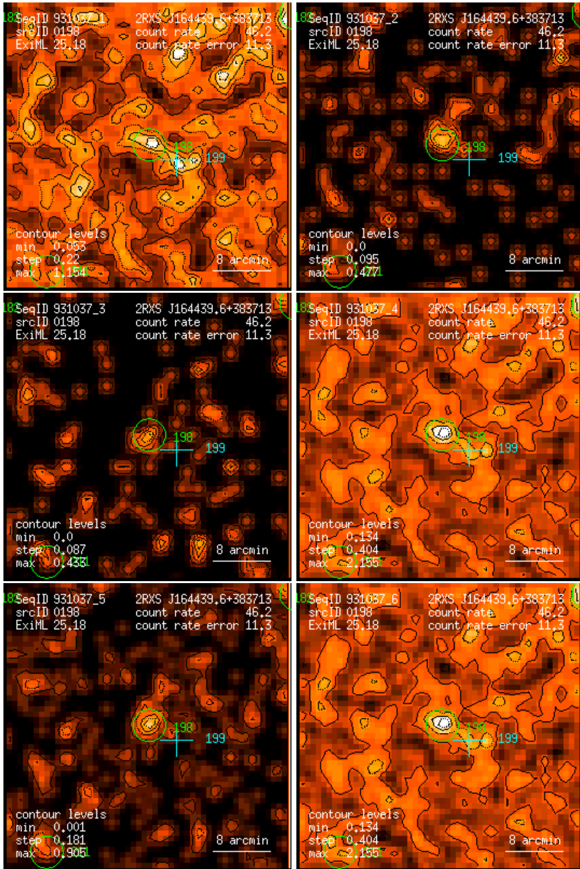
Figure 198: RASS 931037: detection 0198: band rate images, Gaussian filter: (1) PSPC channels 11 – 41, (2) 52 – 90, (3) 91 – 201, (4) 11 – 235, (5) 52 – 201, (6) 11 – 201. Broad band rates in counts/ks. Band rate contour levels in counts/ks/arcmin 2 .
