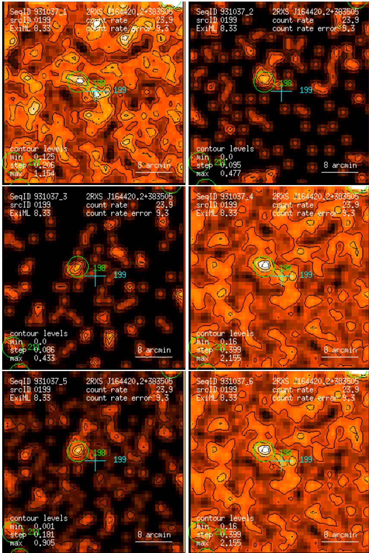
Figure 199: RASS 931037: detection 0199: band rate images, Gaussian filter: (1) PSPC channels 11 – 41, (2) 52 – 90, (3) 91 – 201, (4) 11 – 235, (5) 52 – 201, (6) 11 – 201. Broad band rates in counts/ks. Band rate contour levels in counts/ks/arcmin 2 .
