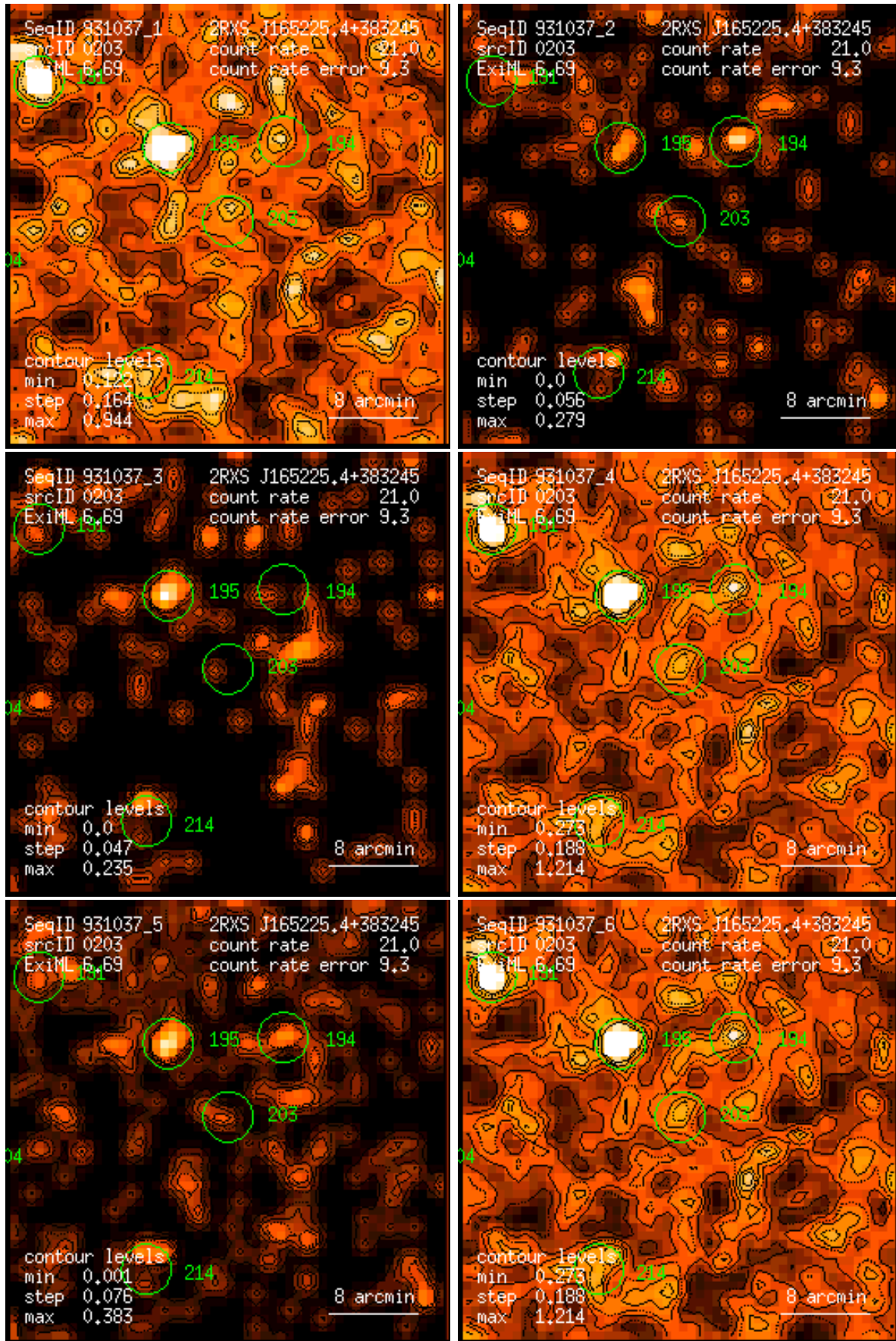
Figure 203: RASS 931037: detection 0203: band rate images, Gaussian filter: (1) PSPC channels 11 – 41, (2) 52 – 90, (3) 91 – 201, (4) 11 – 235, (5) 52 – 201, (6) 11 – 201. Broad band rates in counts/ks. Band rate contour levels in counts/ks/arcmin 2 .
