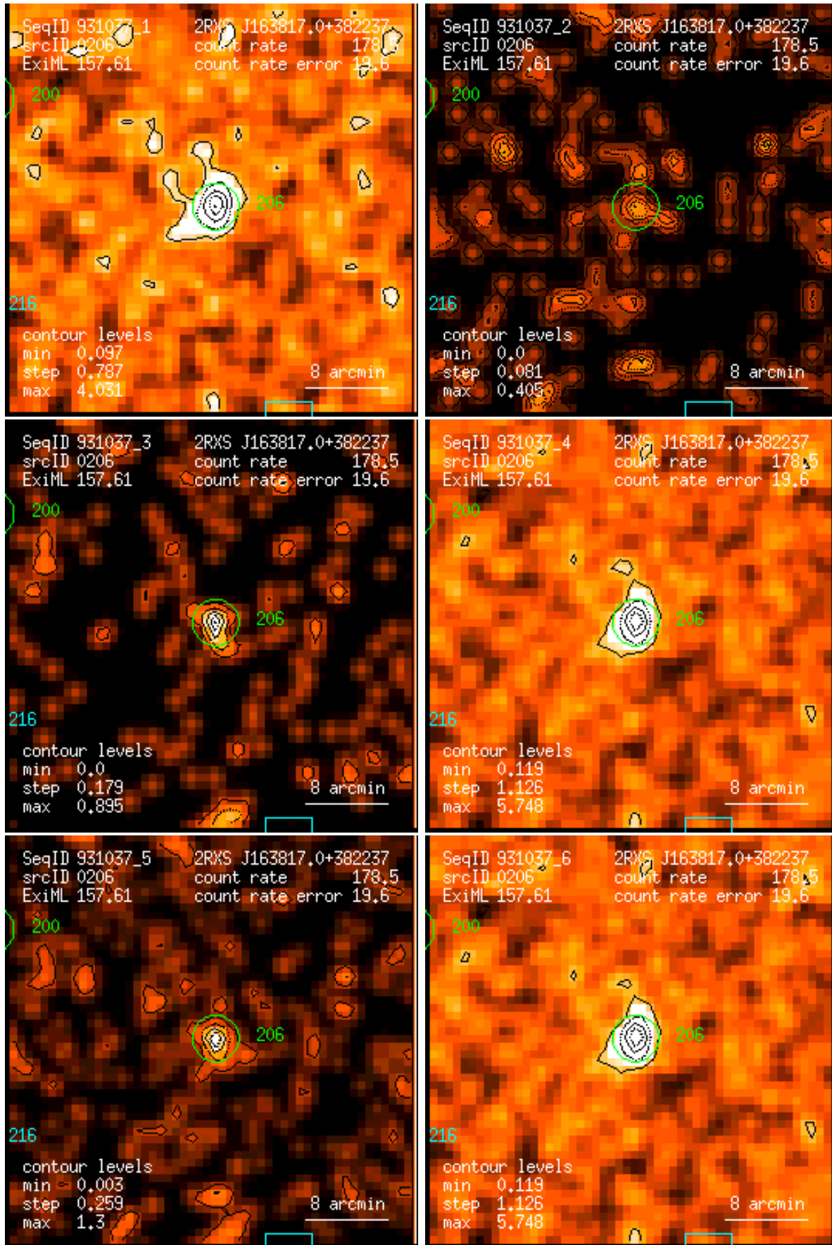
Figure 206: RASS 931037: detection 0206: band rate images, Gaussian filter: (1) PSPC channels 11 – 41, (2) 52 – 90, (3) 91 – 201, (4) 11 – 235, (5) 52 – 201, (6) 11 – 201. Broad band rates in counts/ks. Band rate contour levels in counts/ks/arcmin 2 .
