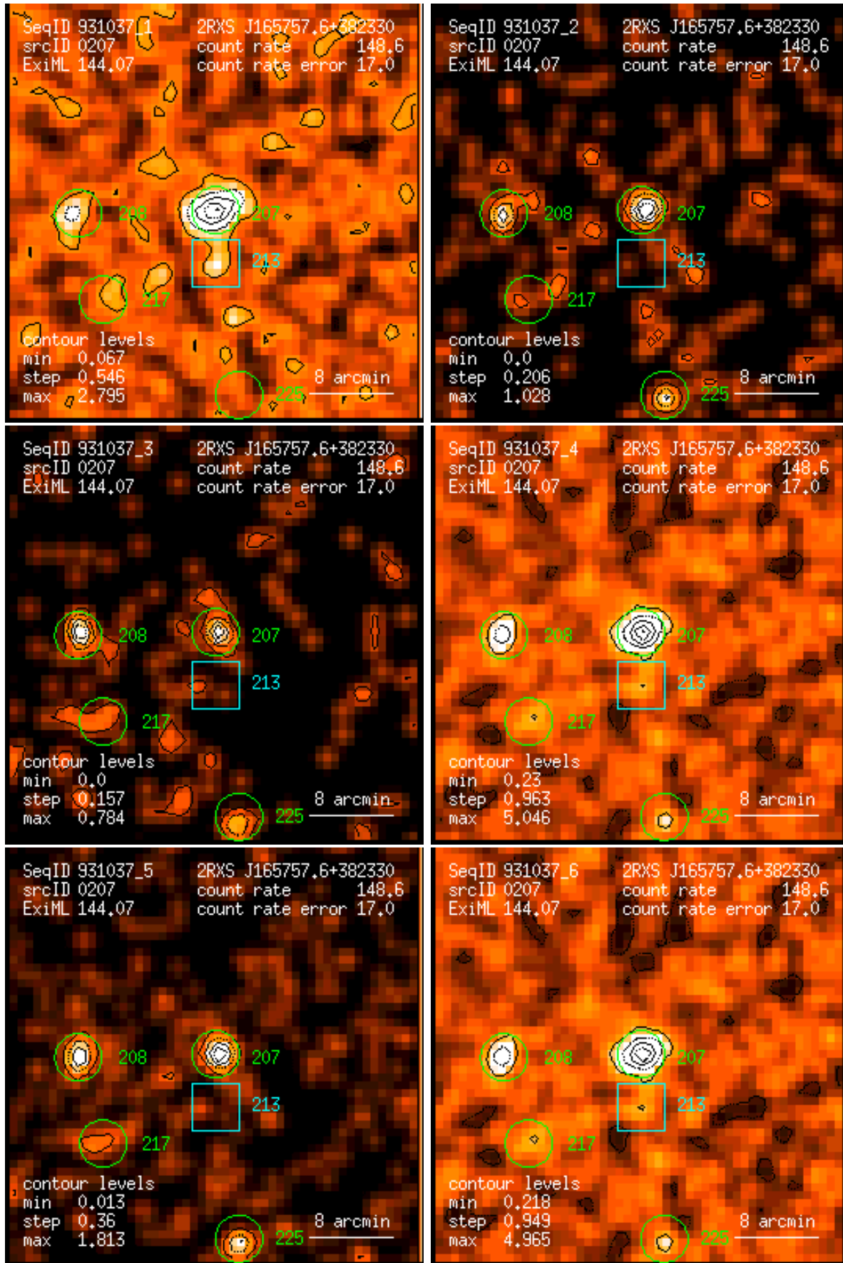
Figure 207: RASS 931037: detection 0207: band rate images, Gaussian filter: (1) PSPC channels 11 – 41, (2) 52 – 90, (3) 91 – 201, (4) 11 – 235, (5) 52 – 201, (6) 11 – 201. Broad band rates in counts/ks. Band rate contour levels in counts/ks/arcmin 2 .
