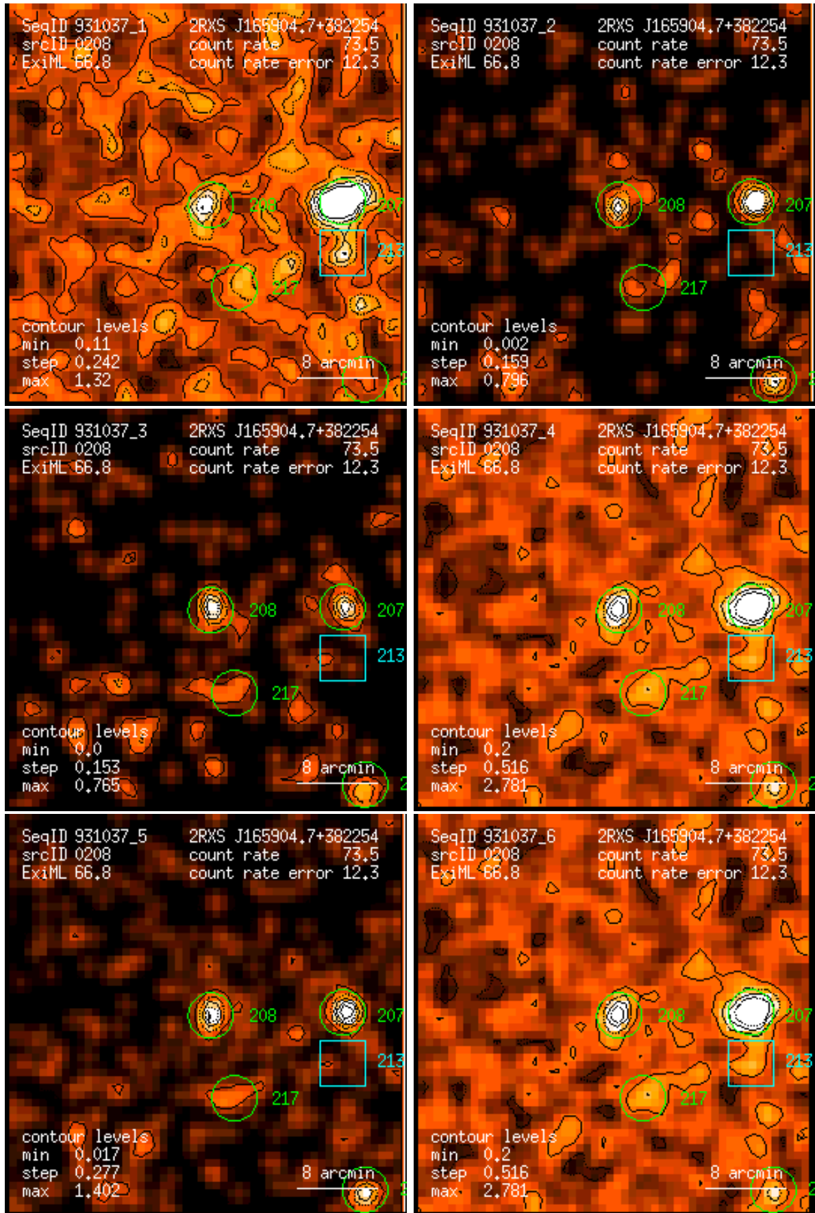
Figure 208: RASS 931037: detection 0208: band rate images, Gaussian filter: (1) PSPC channels 11 – 41, (2) 52 – 90, (3) 91 – 201, (4) 11 – 235, (5) 52 – 201, (6) 11 – 201. Broad band rates in counts/ks. Band rate contour levels in counts/ks/arcmin 2 .
