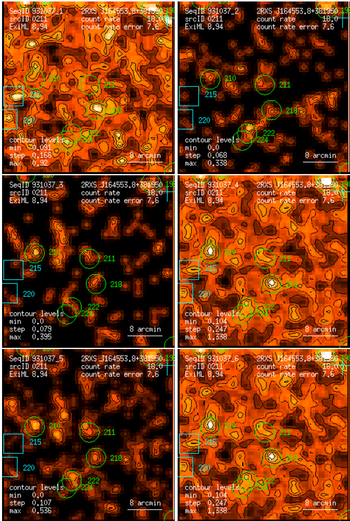
Figure 211: RASS 931037: detection 0211: band rate images, Gaussian filter: (1) PSPC channels 11 – 41, (2) 52 – 90, (3) 91 – 201, (4) 11 – 235, (5) 52 – 201, (6) 11 – 201. Broad band rates in counts/ks. Band rate contour levels in counts/ks/arcmin 2 .
