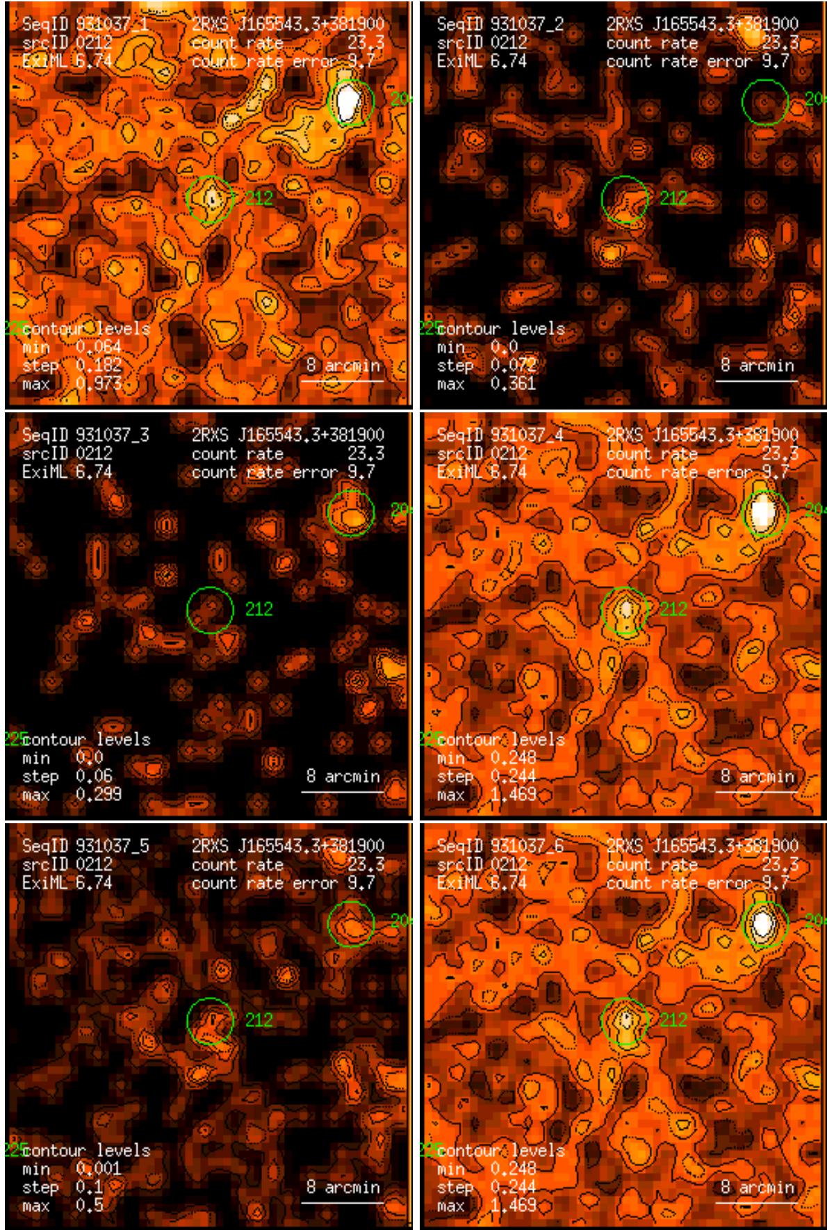
Figure 212: RASS 931037: detection 0212: band rate images, Gaussian filter: (1) PSPC channels 11 – 41, (2) 52 – 90, (3) 91 – 201, (4) 11 – 235, (5) 52 – 201, (6) 11 – 201. Broad band rates in counts/ks. Band rate contour levels in counts/ks/arcmin 2 .
