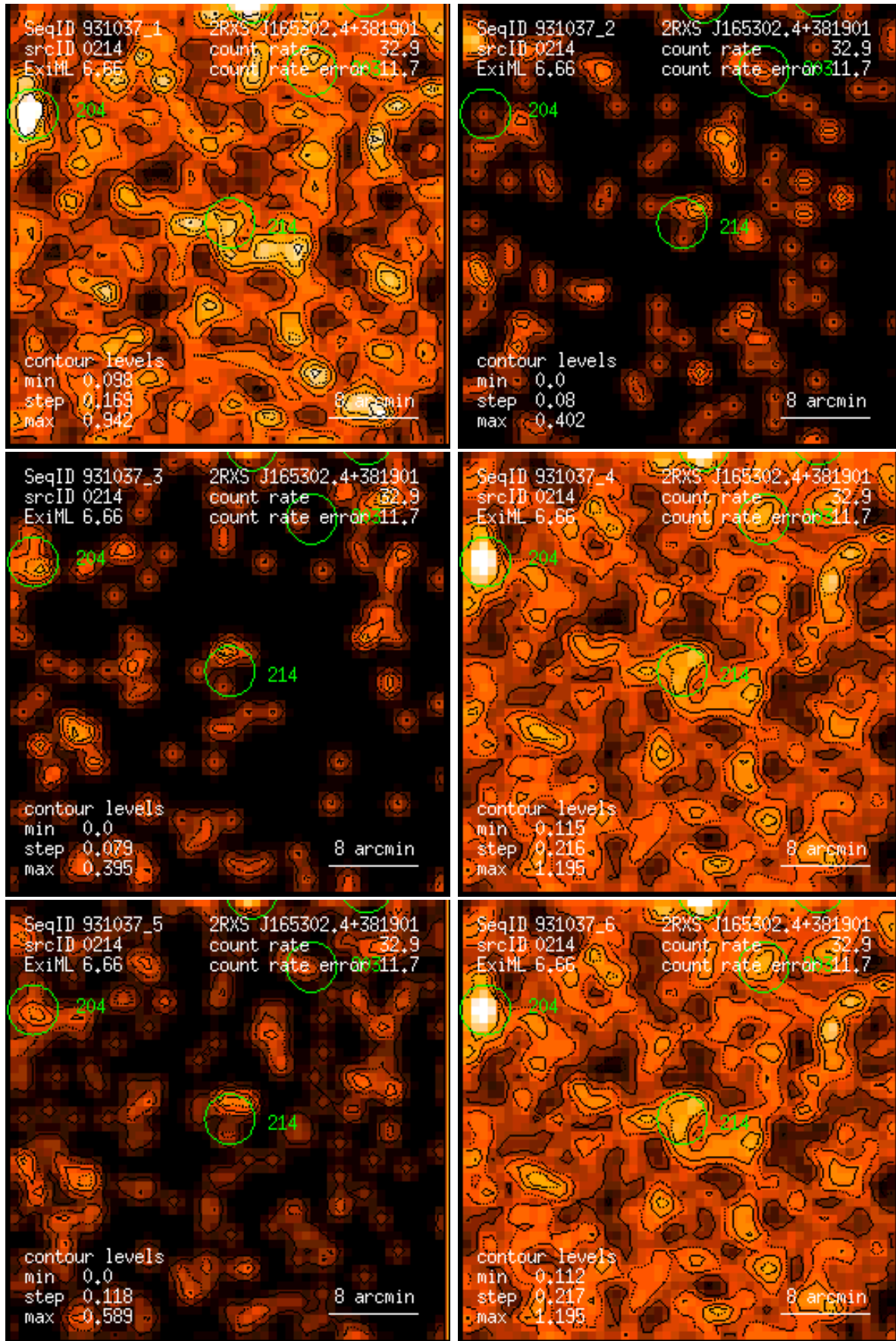
Figure 214: RASS 931037: detection 0214: band rate images, Gaussian filter: (1) PSPC channels 11 – 41, (2) 52 – 90, (3) 91 – 201, (4) 11 – 235, (5) 52 – 201, (6) 11 – 201. Broad band rates in counts/ks. Band rate contour levels in counts/ks/arcmin 2 .
