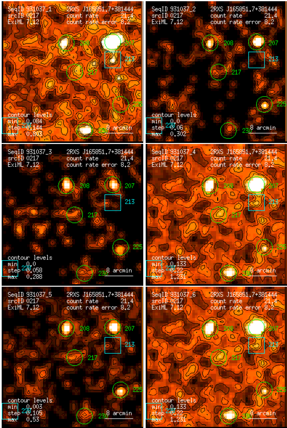
Figure 217: RASS 931037: detection 0217: band rate images, Gaussian filter: (1) PSPC channels 11 – 41, (2) 52 – 90, (3) 91 – 201, (4) 11 – 235, (5) 52 – 201, (6) 11 – 201. Broad band rates in counts/ks. Band rate contour levels in counts/ks/arcmin 2 .
