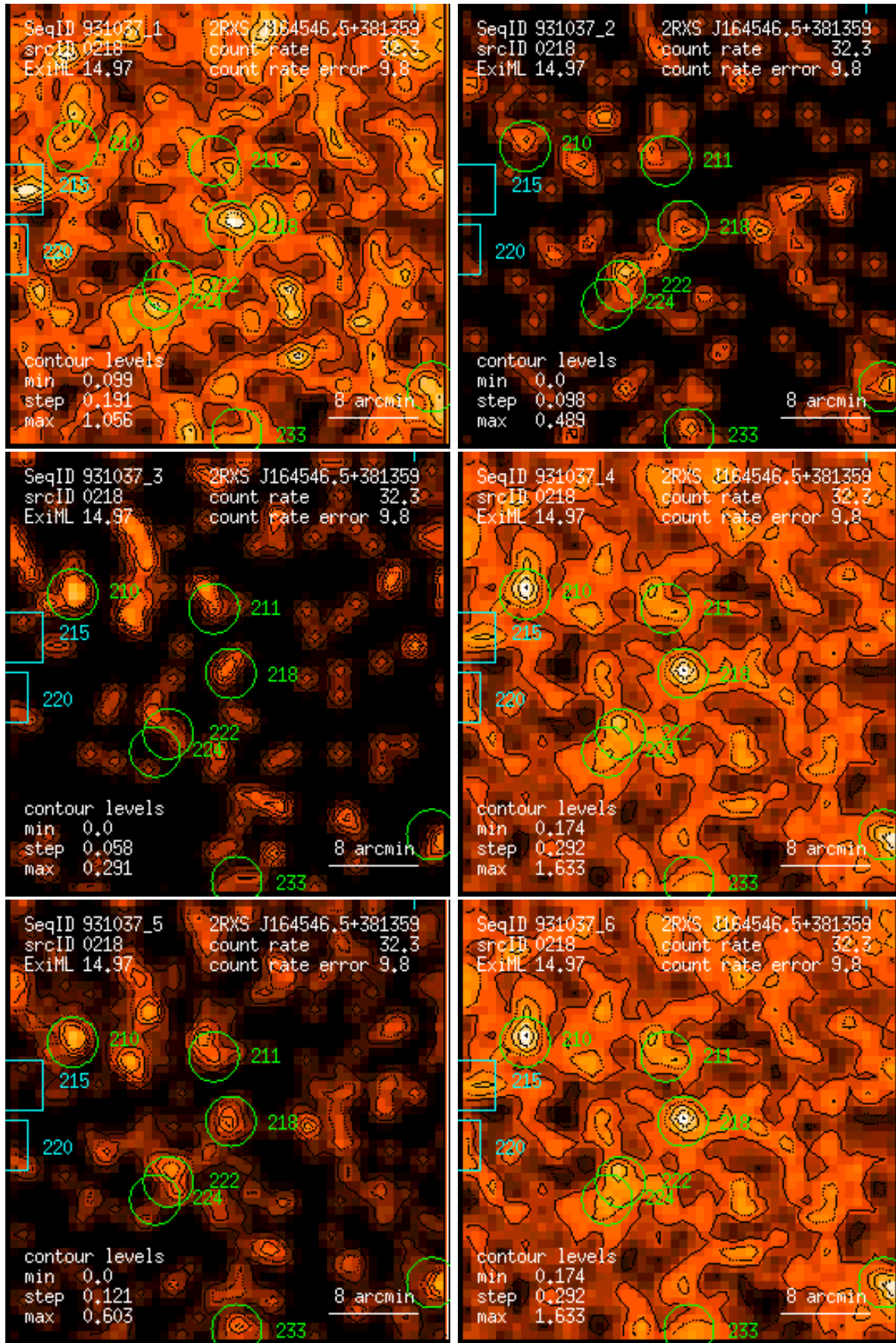
Figure 218: RASS 931037: detection 0218: band rate images, Gaussian filter: (1) PSPC channels 11 – 41, (2) 52 – 90, (3) 91 – 201, (4) 11 – 235, (5) 52 – 201, (6) 11 – 201. Broad band rates in counts/ks. Band rate contour levels in counts/ks/arcmin 2 .
