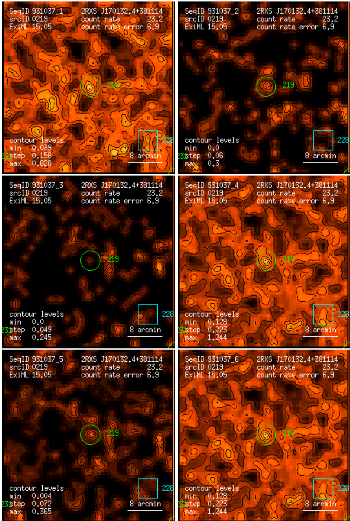
Figure 219: RASS 931037: detection 0219: band rate images, Gaussian filter: (1) PSPC channels 11 – 41, (2) 52 – 90, (3) 91 – 201, (4) 11 – 235, (5) 52 – 201, (6) 11 – 201. Broad band rates in counts/ks. Band rate contour levels in counts/ks/arcmin 2 .
