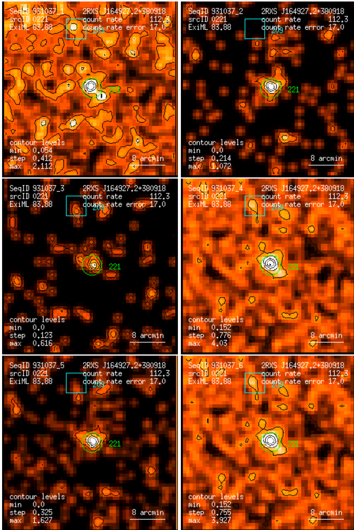
Figure 221: RASS 931037: detection 0221: band rate images, Gaussian filter: (1) PSPC channels 11 – 41, (2) 52 – 90, (3) 91 – 201, (4) 11 – 235, (5) 52 – 201, (6) 11 – 201. Broad band rates in counts/ks. Band rate contour levels in counts/ks/arcmin 2 .
